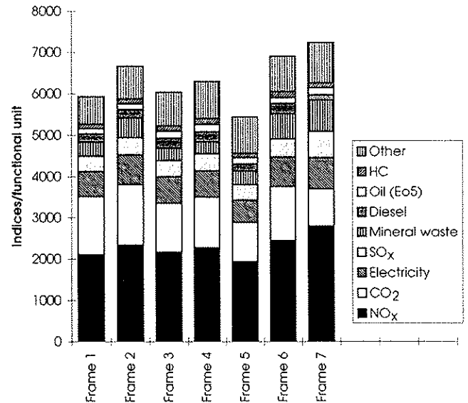
Fig. 8: Environmental impact per functional unit for seven frames for building production from cradle to gate (Step 1) when applying the Environmental theme method
