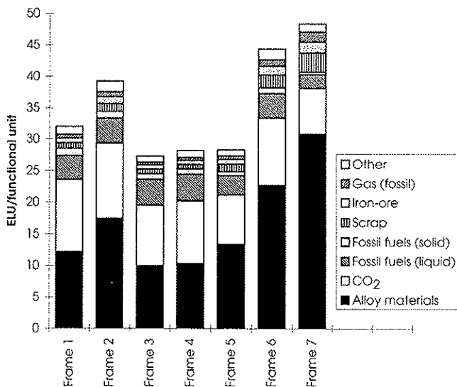
Fig. 7: Environmental impact per functional unit for seven frames for building production from cradle to gate (Step 1) when applying the EPS method
