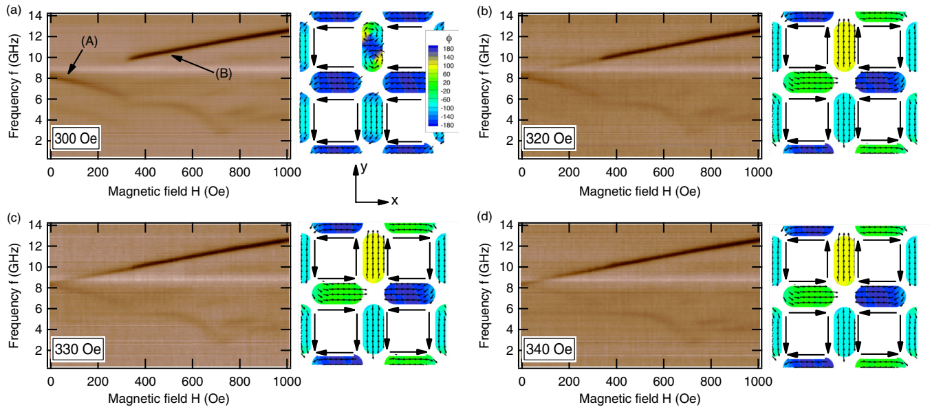
FIG. 4. Observation of FMR spectra in the low magnetic field regime. After saturating at -3100 Oe, the initialization field H_{\text{ini}} is applied and then the spectrum is recorded starting at 0 Oe while gradually increasing the applied field. (a)–(d) H_{\text{ini}} was varied from 300 Oe to 340 Oe. At 300 Oe, the modes (A) and (B) do not coexist at zero field, (a), but as the field increases mode (B) appears at lower fields, (b) and (c). Increasing H_{\text{ini}} beyond 330 Oe leads to a disappearance of (A) at H = 0 Oe, (d). The static equilibrium magnetization states at zero field are shown next to each spectrum. The color coding indicates the azimuthal in-plane angle of the magnetization. The arrows next to each island indicate the average magnetization direction in the island.
