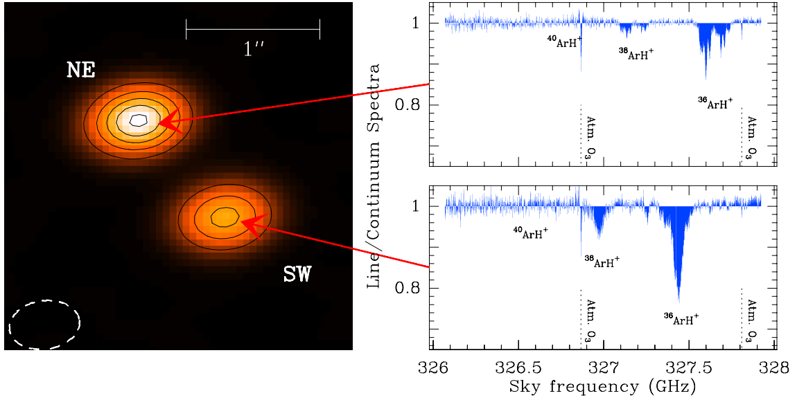
Fig. A.1. Map of the 339 GHz continuum emission of PKS 1830–211 showing the two resolved lensed images of the blazar ( left ). Overview of the ArH + absorption spectrum toward PKS 1830–211 SW ( bottom right ) and NE ( top right ) from the current observations. Expected positions of the main absorption feature are indicated for 36 ArH + , 38 ArH + , and 40 ArH + ; the last is not detected. The noise increases toward lower frequencies because of the proximity of the atmospheric water line near 325.2 GHz.
