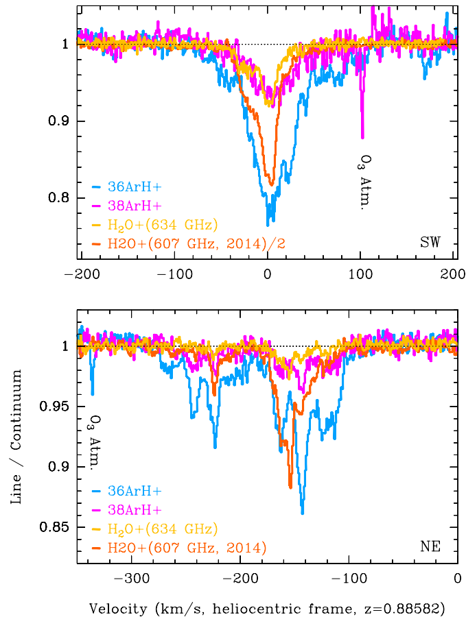
Fig. 1. Spectra of 36 ArH + and 38 ArH + toward PKS 1830–211 SW ( top ) and NE ( bottom ) images, together with two para -H 2 O + fine structure lines of the 1_{10}-1_{01} transition; none of the transitions shows hyperfine splitting.
