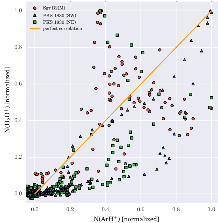
Fig. A.2. Normalized correlation plot of H 2 O + versus 36 ArH + toward PKS 1830–211 SW, NE, and Sagittarius B2(M). The column densities of the two species have been normalized by the maximum values for each component and for each velocity channel. A perfect correlation (i.e. just a constant scaling factor between the two species) would result in clustering along the yellow line. The distributions of the two cations are poorly correlated toward the sources. The PKS 1830–211 data are from this work and from Müller et al. (in prep.) for 36 ArH + and H 2 O + , respectively; the corresponding Sagittarius B2(M) data are from Schilke et al. (2014) and Schilke et al. (2013).
