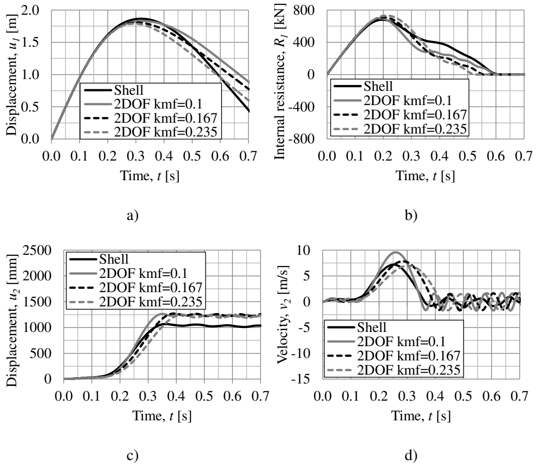
Figure C.36 Illustration of collision J8, a) displacement of body 1 u_1 , b) internal resistance of body 1 R_1 , c) displacement of body 2 u_2 , and d) velocity of body 2 v_2 .
