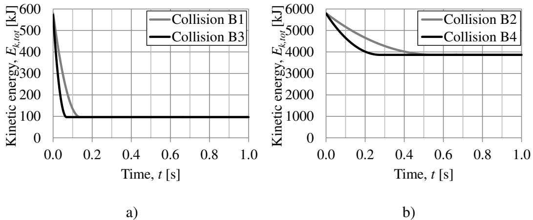
Figure 3.10 Change in kinetic energy E_{k,tot} in the positive direction of body 2 during a) collision B1 and B3, and b) collision B2 and B4.
