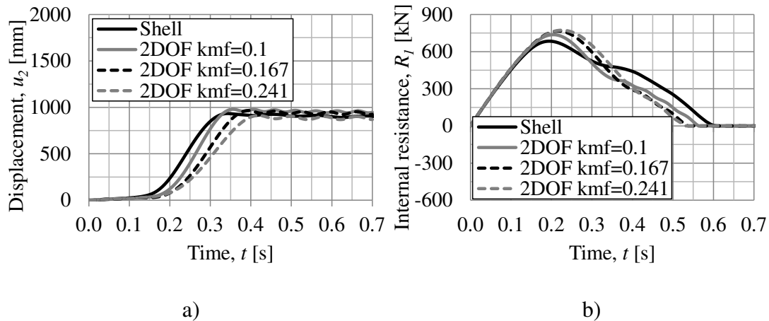
Figure 6.44 Illustration of the response for collision J9 with R_{2,max} obtained from the FE analysis as input data, a) displacement of body 2, and b) internal resistance of body 1 R_1 .
