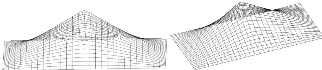
Figure 6.23 Illustration of the element grid and the deformation of the beam grillage model in ADINA from two different angles of view.
