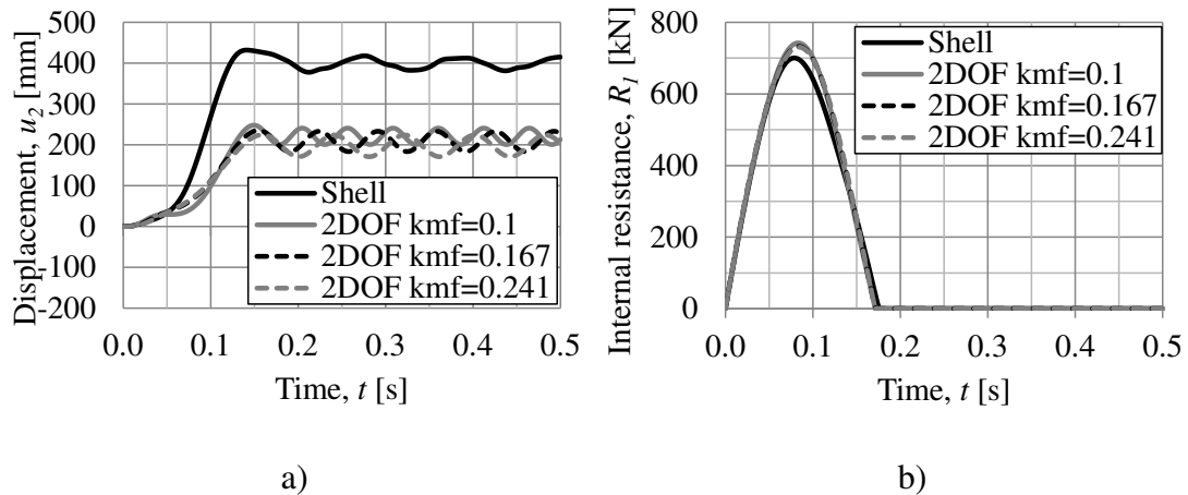
Figure 6.41 Illustration of the response for collision J3 with R_{2,max} obtained from the FE analysis as input data, a) displacement of body 2, and b) internal resistance of body 1 R_1 .
