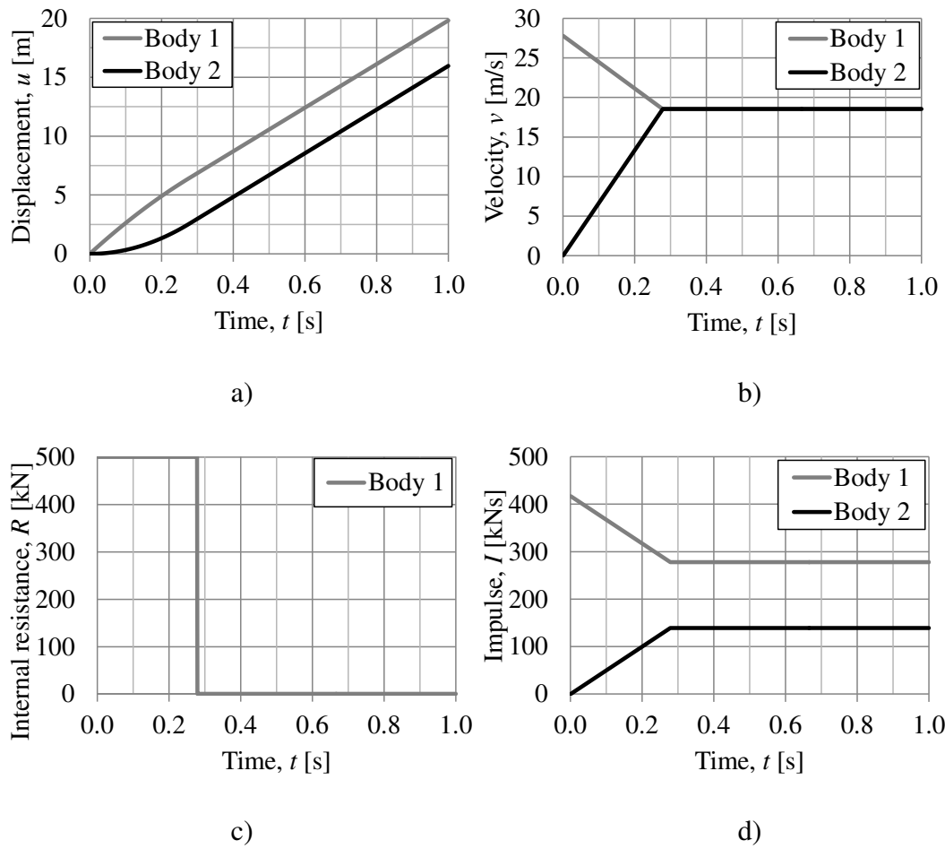
Figure B.9 Response for collision B4 a) displacement u , b) velocity v , c) internal resistance R , and d) impulse I .
