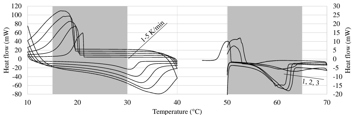
Fig. 1. DSC measurement results for a sample of ClimSel C24 (left) depending on the rate of heating and cooling and three samples of ClimSel C58 (right). The gray square marks the storage temperature range according to the product declarations [4].
