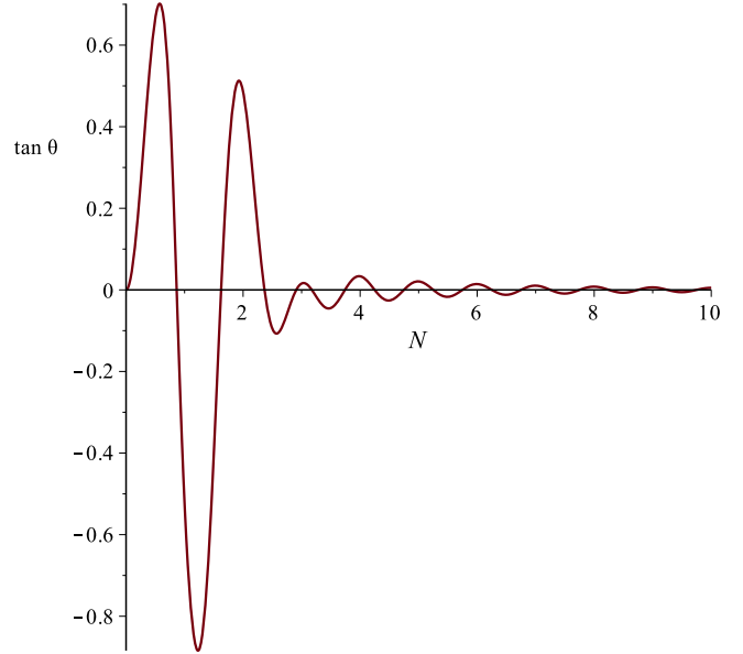
FIG. 3. (Color online) \tan \theta_{\text{as}} from Eq. (46) as a function of pulse duration N for K = 2 and a_0 = 2 . [Note that in the absence of RR this tangent would be infinite for any N as the asymptotic emission angle is \pi/2 in this case; cf. Fig. 11 below.]
