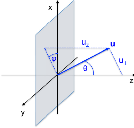
FIG. 1. (Color online) Sketch of the ejection geometry with the laser propagating in z direction. \theta and \varphi are polar and azimuthal ejection angles, respectively. \mathbf{u} denotes the spatial part of the electron four-velocity.
