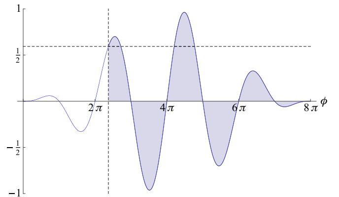
FIG. 2. (Color online) Sketch of the field of a laser pulse. The horizontal dashed line represents the ionization threshold. Only the shaded region contributes to the integral Eq. (3) determining the electron ejection angle.
