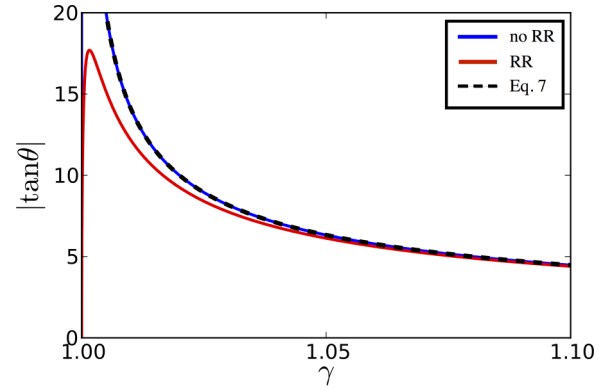
FIG. 11. (Color online) Numerical result for the correlation between final emission angle and \gamma , for a_0 = 200 , \sin^4 envelope. Blue (top) curve: Lorentz force; see Ref. [1]. Red (bottom) curve: RR result. The black (dashed) line corresponds to Eq. (7).
