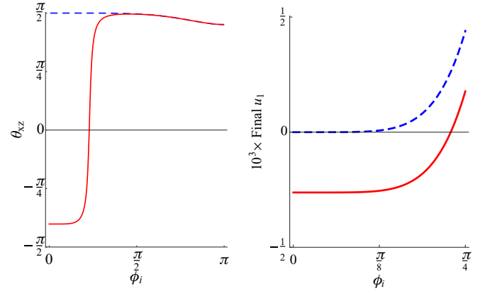
FIG. 6. (Color online) Left: Planar angle \theta_{xz} , for N = 4 cycles of an a_0 = 50 pulse with \sin^4 envelope. Right: final transverse velocity, as a function of \phi_i . The sign flip in the transverse component, for \phi_i \lesssim \pi/4 , is responsible for the large change in emission angle. Blue (dashed): Lorentz case; red (solid): RR.
