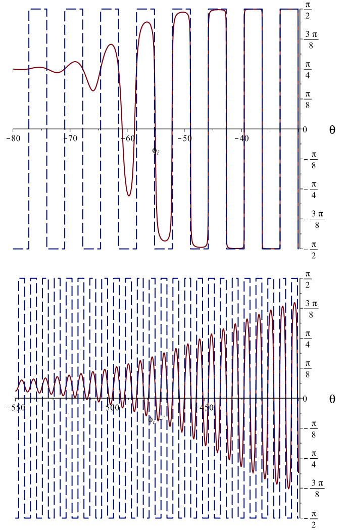
FIG. 9. (Color online) \theta_L [blue (dashed)] and \theta_{\text{RR}} [red (solid)] as functions of ionization phase \phi_i for the pulse Eq. (50) with (top panel) N = 4 , a_0 = 5 and (bottom panel) N = 40 , a_0 = 50 .
