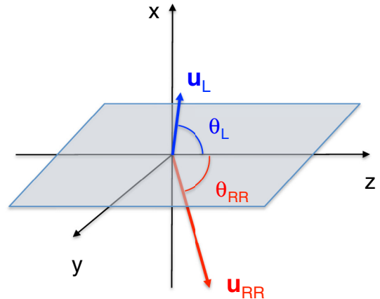
FIG. 7. (Color online) Qualitative sketch (not to scale) of the reversal in ejection direction due to RR (red, subscript RR) as compared to the Lorentz case (blue, subscript L).
