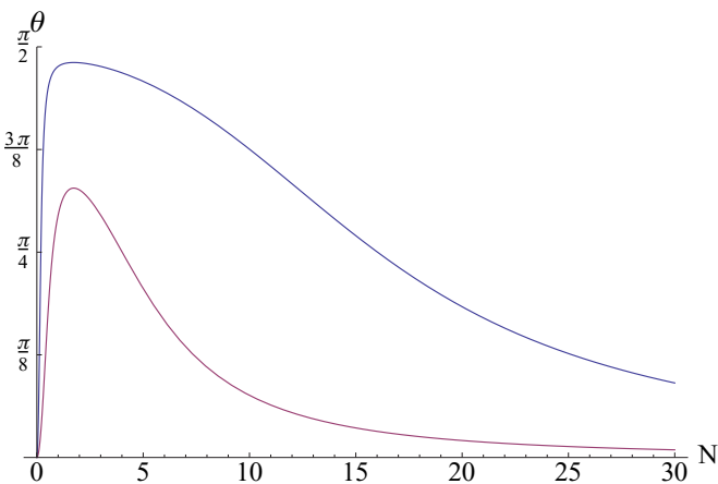
FIG. 8. (Color online) \theta_{\text{as}} from Eq. (51) as a function of pulse duration N for the pulse Eq. (50). Upper curve: a_0 = 50 , lower curve: a_0 = 5 .
