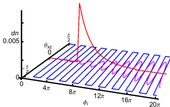
FIG. 10. (Color online) Horizontal plane: Planar ejection angle \theta_{xz} for N = 1\,600 , a_0 = 10 , \sin^2 envelope, as a function of ionization time \phi_i , for Lorentz [blue (rectangular)] and RR [magenta (rounded)]. Note the difference in ejection angle between pure Lorentz and RR scenarios. Vertical direction: Ionization rate dn as defined in the main text.
