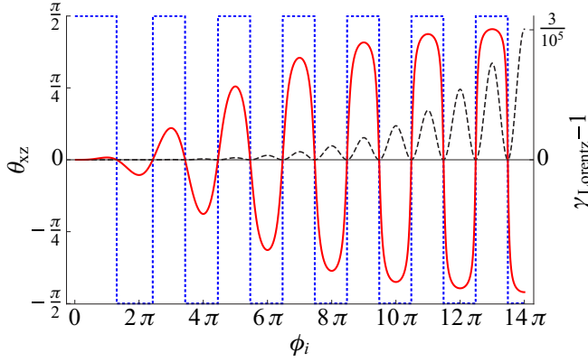
FIG. 5. (Color online) Left scale: planar angle \theta_{xz} for N = 1600 , a_0 = 10 , \sin^2 envelope, as a function of ionization time \phi_i , for Lorentz [blue (dotted)] and RR [red (solid)]. Right: final Lorentz force \gamma for the emitted particles [black (dashed)].
