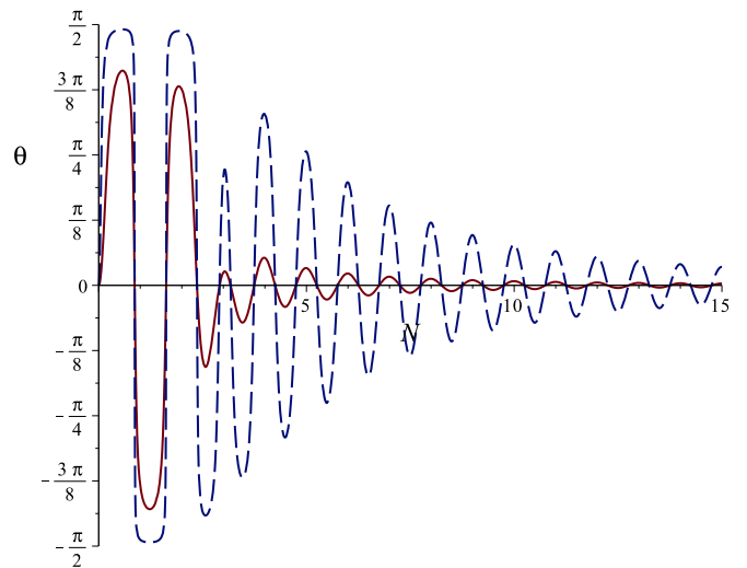
FIG. 4. (Color online) Emission angle \theta_{\text{RR}} as a function of pulse duration N for K = 2 and a_0 = 5 [red (solid)] and a_0 = 50 [blue (dashed)].
