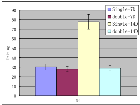
Figure 17 The ions mass caught by passive samplers in the simulation experiment of synthetic fresh water medium
