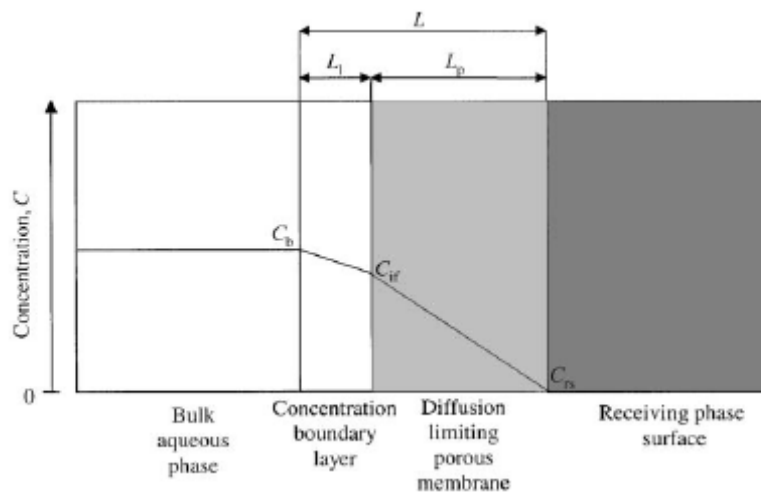
Figure 4 Diagrammatic representation of the diffusion path for analytes from the bulk aqueous phase to the surface of the receiving phase in the passive sampler.
