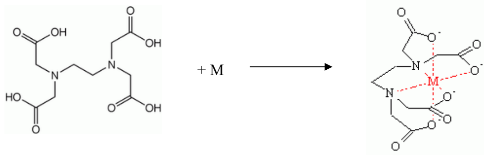
Figure 5 The formation of metal-EDTA complex
