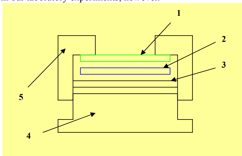
Figure 1 Cross-section of the passive sampler: 1 diffusion limiting porous membrane, 2 receiving membrane, 3 polypropylene supporting disk, 4 polypropylene screw lid, 5 polypropylene body.
