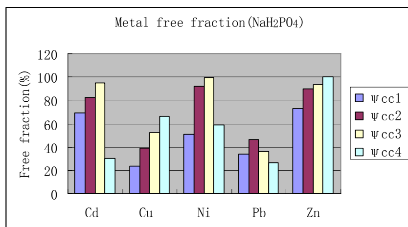
Figure 12 Metal free fractions in NaH 2 PO 4 beaker experiment; \psi_{cc1} : \psi_{cc} of beaker 1; \psi_{cc2} : \psi_{cc} of beaker 2; \psi_{cc3} : \psi_{cc} of beaker 3; \psi_{cc4} : \psi_{cc} of beaker 4.
