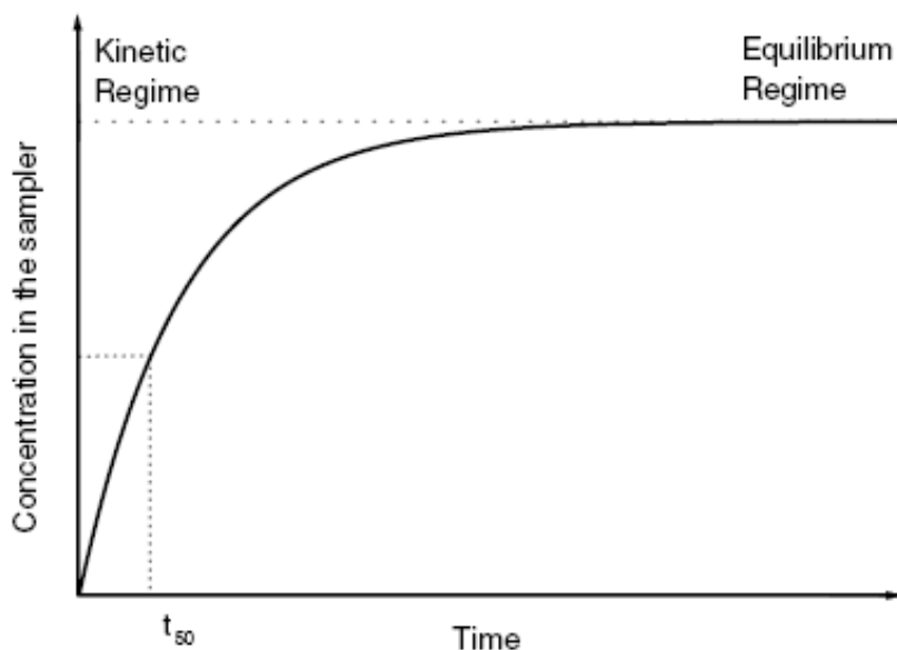
Figure 3 Passive sampling devices operate in two main regimes (kinetic and equilibrium).
