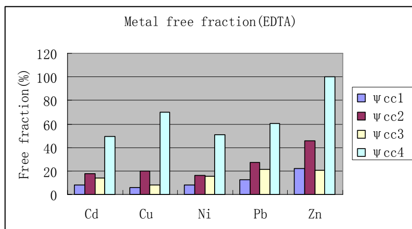
Figure 11 Metal free fractions in EDTA beaker experiment; \psi_{cc1} : \psi_{cc} of beaker 1; \psi_{cc2} : \psi_{cc} of beaker 2; \psi_{cc3} : \psi_{cc} of beaker 3; \psi_{cc4} : \psi_{cc} of beaker 4.
