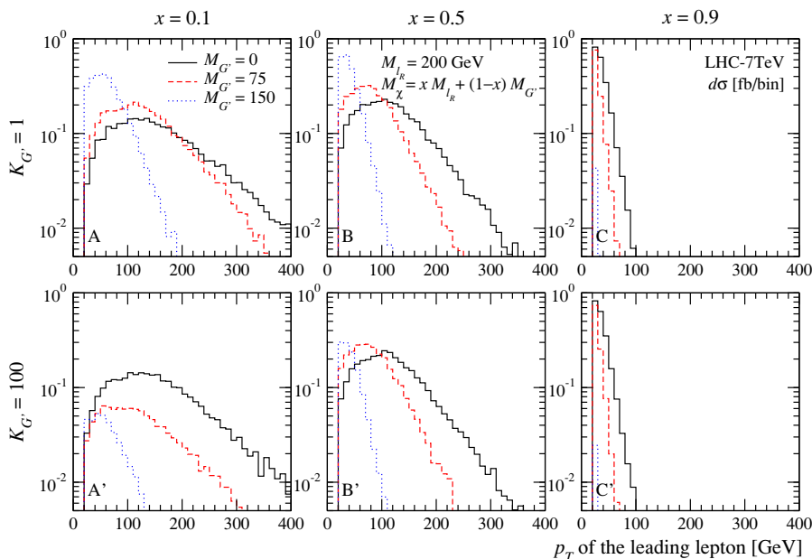
Figure 6. Transverse momentum distributions of the leading lepton for pp \rightarrow \tilde{\ell}_R^+ \tilde{\ell}_R^- \rightarrow \ell^+ \ell^- + \gamma\gamma + \cancel{E}_T at \sqrt{s} = 7 \text{ TeV} for M_{\ell_R} = 200 \text{ GeV} with various neutralino and pseudo-goldstino masses. The value of K_{G'} is fixed at 1 and 100 in the top and bottom figures, respectively.
