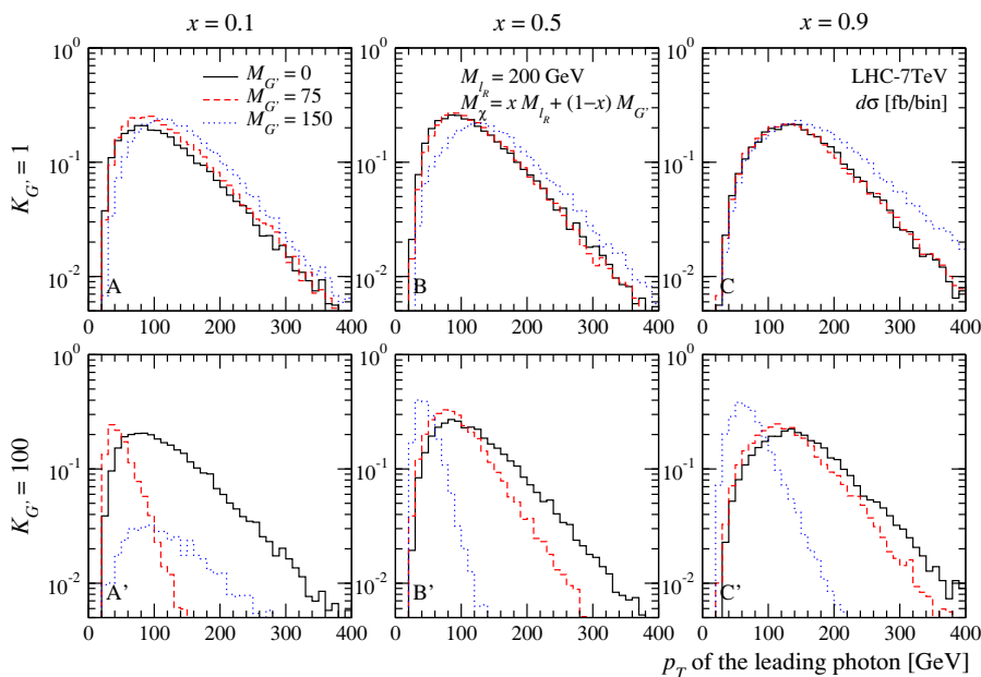
Figure 7. The same as in figure 6, but for the transverse momentum of the leading photon.
