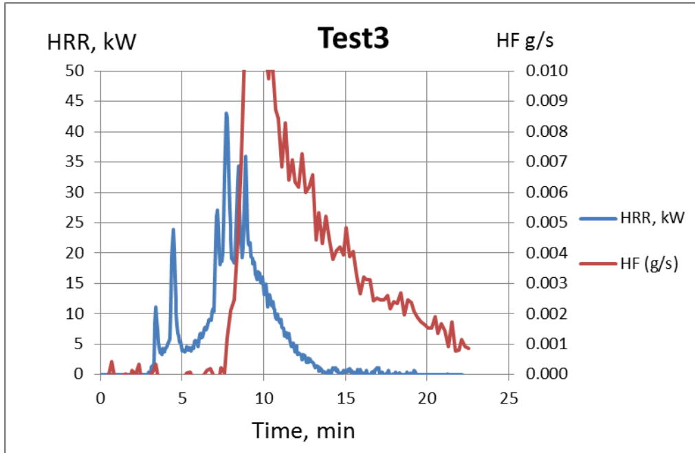
Figure 68 HRR and HF production as a function of time for test 3. The HF production only includes the readout from the FTIR so HF that is captured in the filter is not included.
