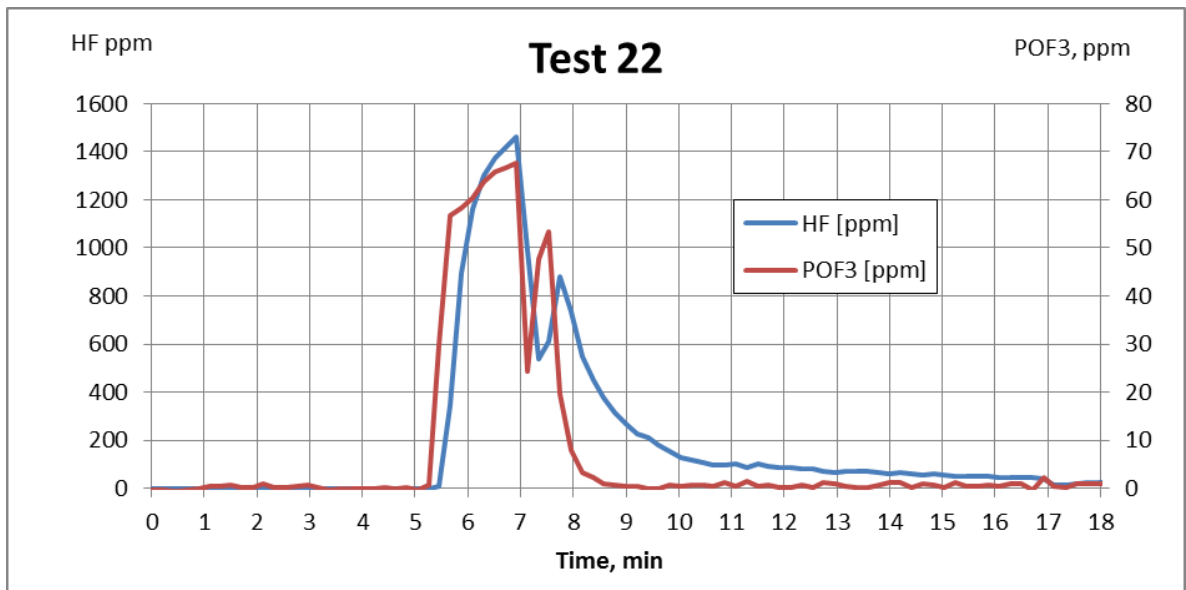
Figure 42 HF and \text{POF}_3 concentration as a function of time for test 22. DMC with salt was injected under time 5-7 minutes.
