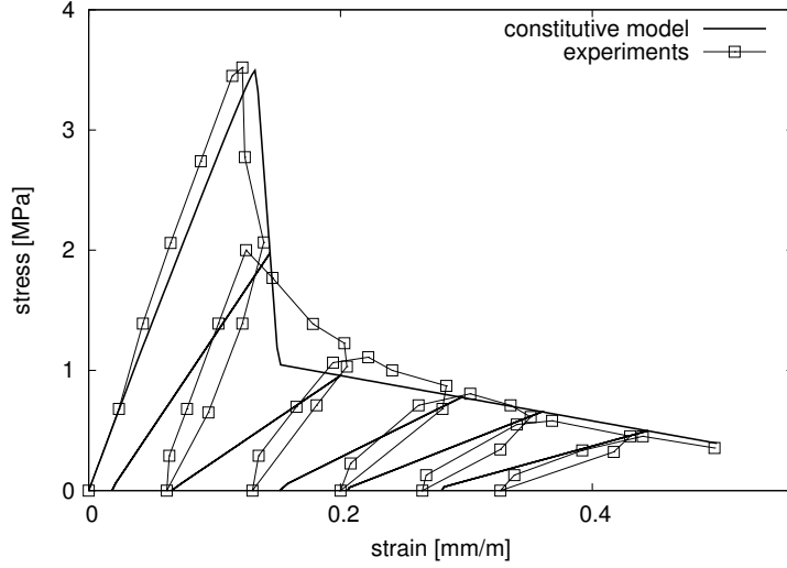
Figure 7: Uniaxial tension: Model response compared to experimental results in Gopalaratnam and Shah (1985).
