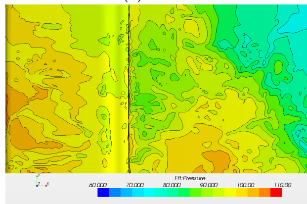
(c) SST-DES
