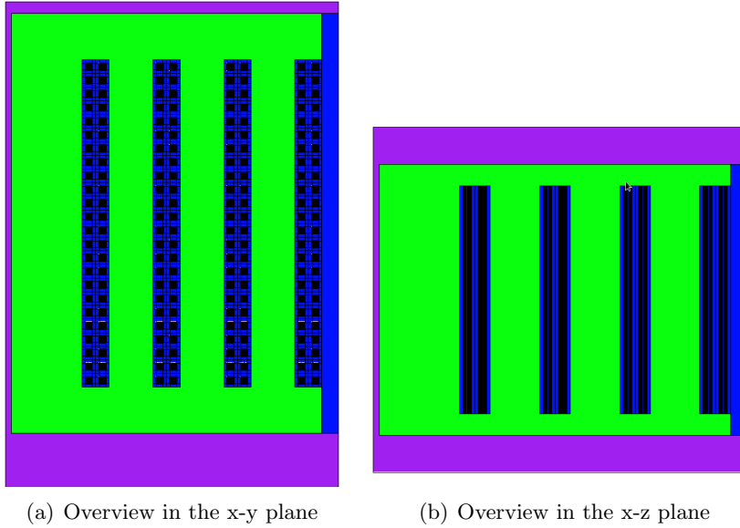
Figure 3.3: Plots of the dry storage facility model for O2 obtained using MCNP
