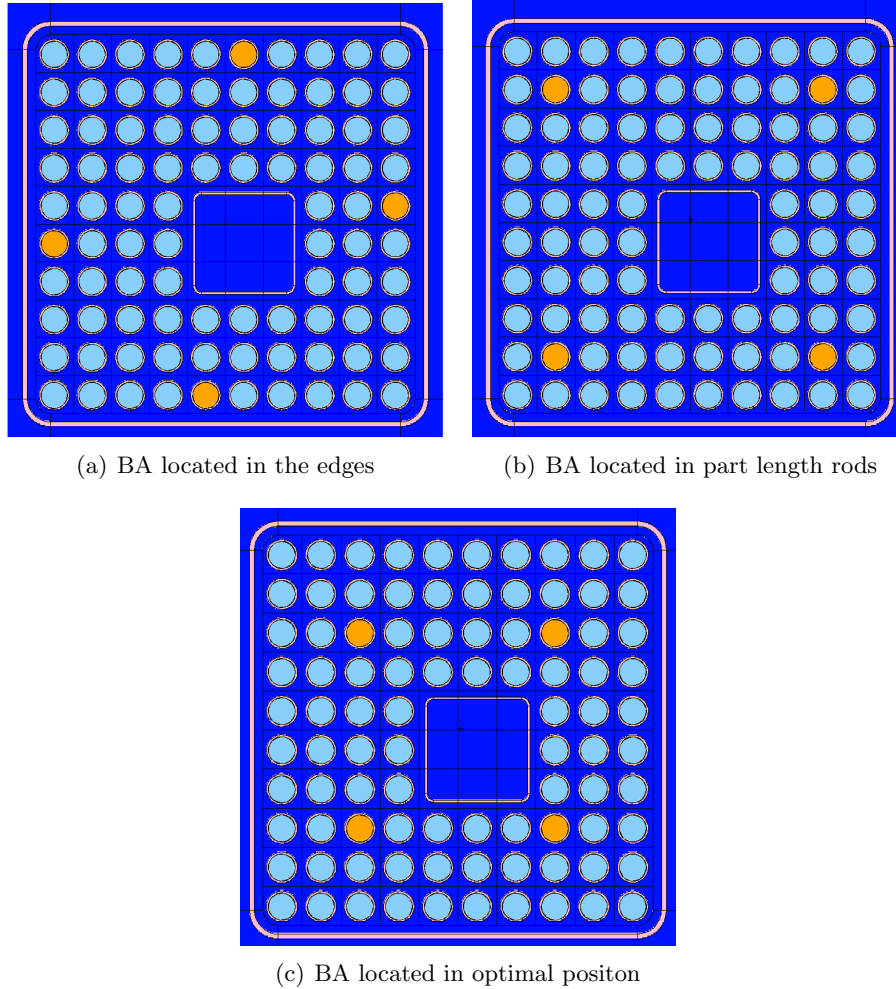
Figure 3.5: Cross section view of the 'Atrium 10XM' fuel bundle design model with Burnable Absorbers in different positions for O2 obtained using MCNP
