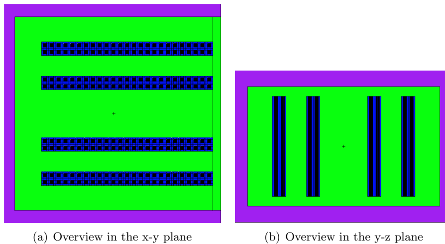
Figure 3.6: Plots of the dry storage facility model for O3 obtained using MCNP
