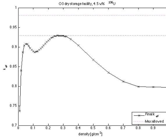
Figure 5.23: Final result of simulations of the O3 facility
