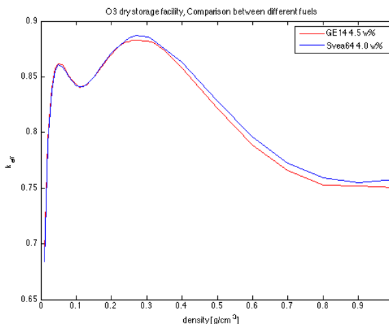
Figure 5.31: Comparison between 'Svea-64' and 'GE-14 Nordic' for the facility O3
