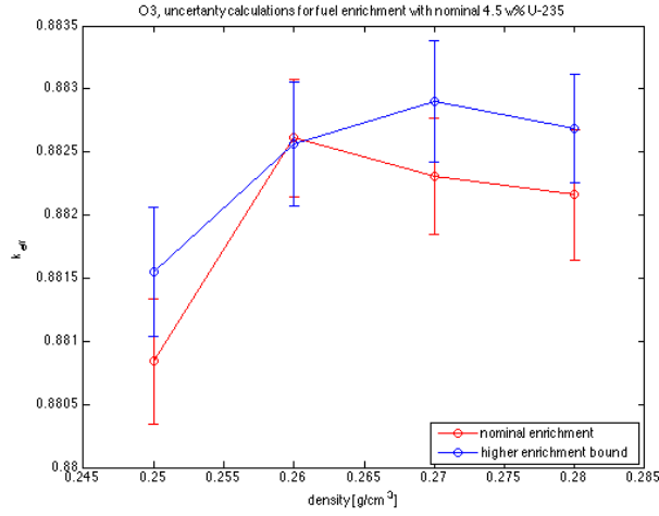
Figure 5.9: Results from simulations around optimal moderation for O3 with vendor supplied uncertainty in enrichment level
