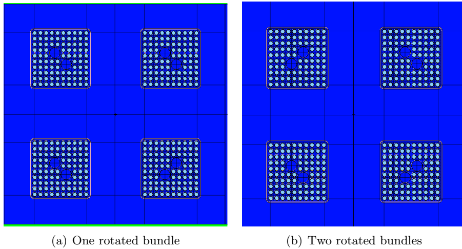
Figure 4.3: Plots of the rotated fuel bundles inside O1/O3 dry storage facility
