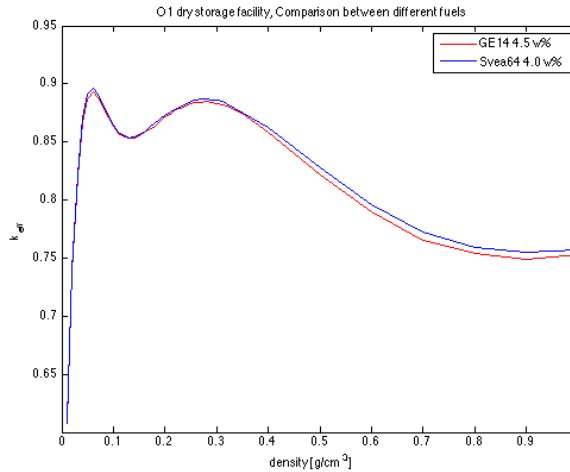
Figure 5.29: Comparison between 'Svea-64' and 'GE-14 Nordic' for the facility O1
