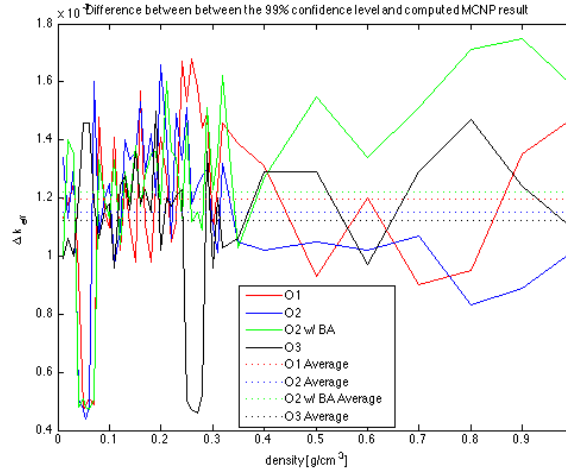
Figure 5.26: Obtained result subtracted from the 99% confidence interval value for each density of the simulations
