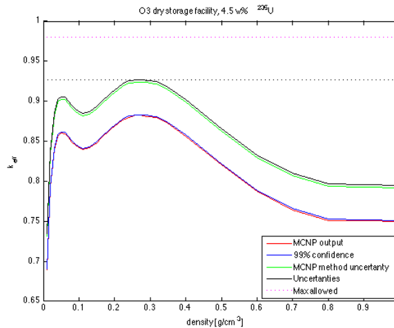
Figure 5.24: Breakdown of final result from simulations of the O3 facility
