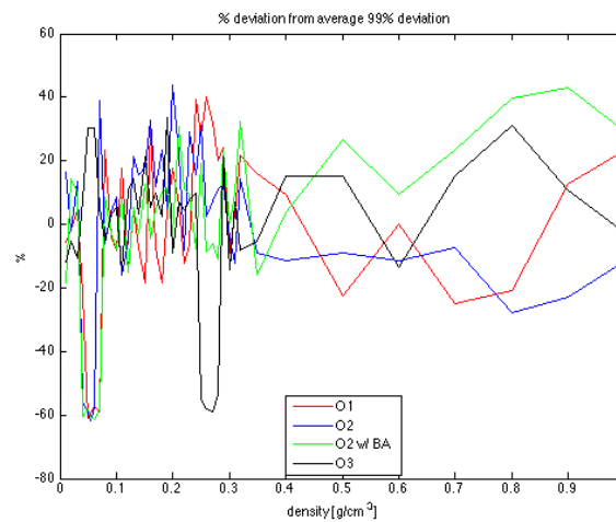
Figure 5.27: Obtained result subtracted from the 99% confidence interval value for each density of the simulations presented as % deviation from the mean value for the facility
