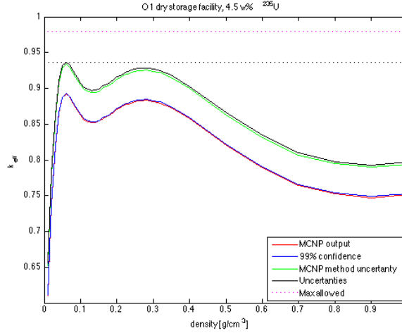
Figure 5.16: Breakdown of final result from simulations of the O1 facility
