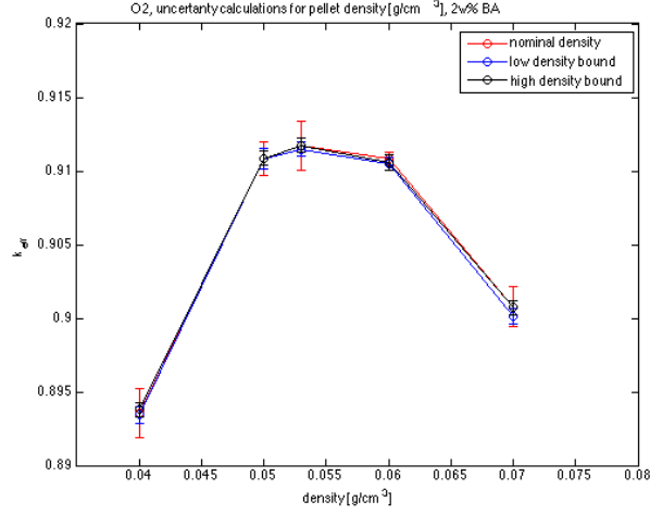
Figure 5.14: Results from simulations around optimal moderation for O2 with vendor supplied uncertainty in BA pellet density
