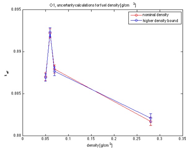
Figure 5.10: Results from simulations around optimal moderation for O1 with vendor supplied uncertainty in pellet density
