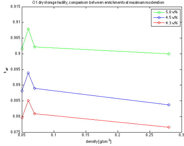
Figure 5.1: Results from simulations around optimal moderation for O1 with different enrichment levels
