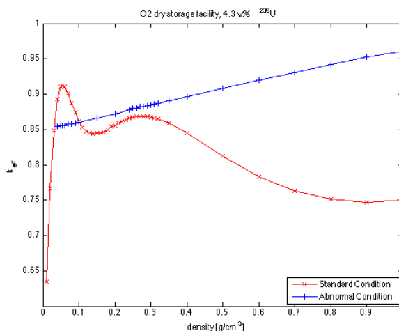
Figure 5.28: Example of a special case where the k_{\text{eff}} can obtain a higher value than allowed
