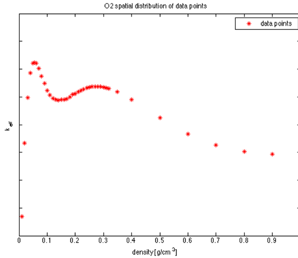
Figure 4.2: Datapoints of the simulations
