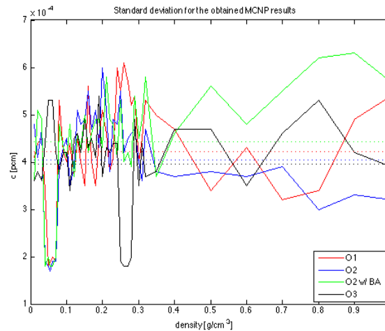
Figure 5.25: Standard deviation of k_{\text{eff}} for each facility as a function of moderator density
