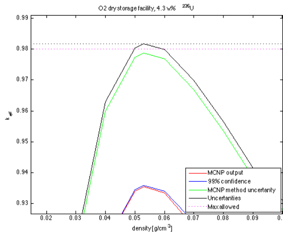
Figure 5.19: Zoom around optimal moderation on breakdown of final result from simulations of the O2 facility without BA present
