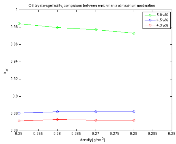
Figure 5.3: Results from simulations around optimal moderation for O3 with different enrichment levels
