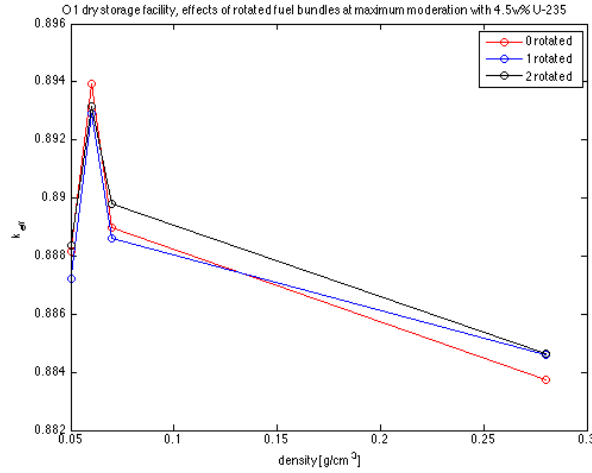
Figure 5.4: Results from simulations around optimal moderation for O1 with rotated fuel bundles
