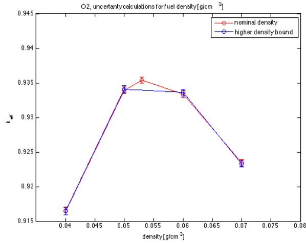
Figure 5.11: Results from simulations around optimal moderation for O2 with vendor supplied uncertainty in pellet density
