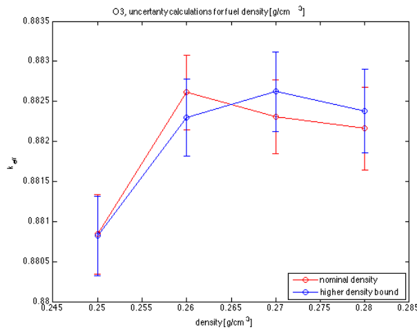
Figure 5.12: Results from simulations around optimal moderation for O3 with vendor supplied uncertainty in pellet density
