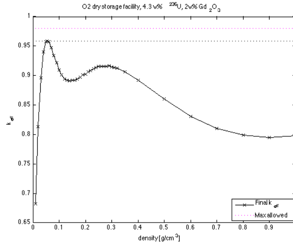
Figure 5.21: Final result of simulations of the O2 facility with BA present
