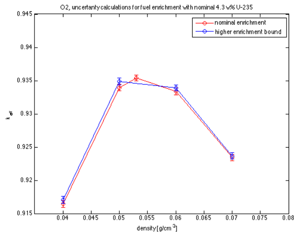
Figure 5.8: Results from simulations around optimal moderation for O2 with vendor supplied uncertainty in enrichment level
