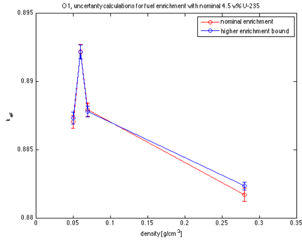
Figure 5.7: Results from simulations around optimal moderation for O1 with vendor supplied uncertainty in enrichment level
