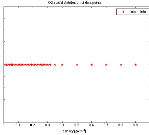
Figure 4.1: The different densities of the simulations
