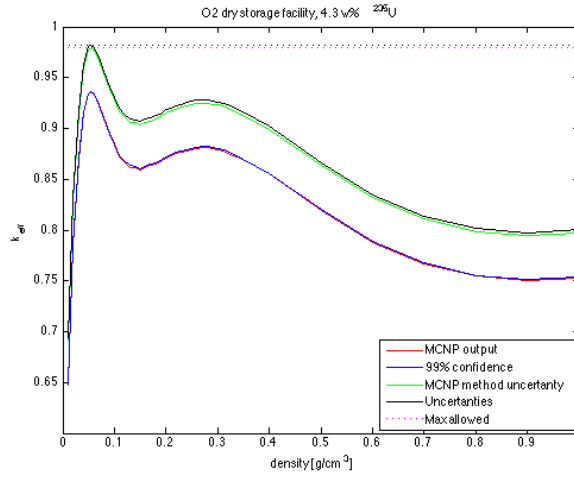
Figure 5.18: Breakdown of final result from simulations of the O2 facility without BA present
