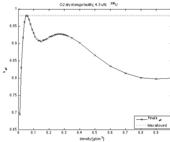
Figure 5.17: Final result of simulations of the O2 facility without BA present
