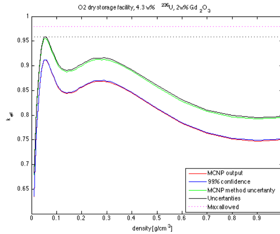
Figure 5.22: Breakdown of final result from simulations of the O2 facility with BA present
