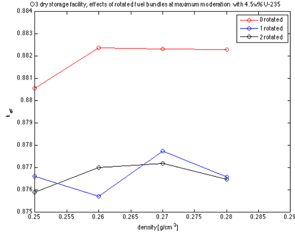
Figure 5.6: Results from simulations around optimal moderation for O3 with rotated fuel bundles
