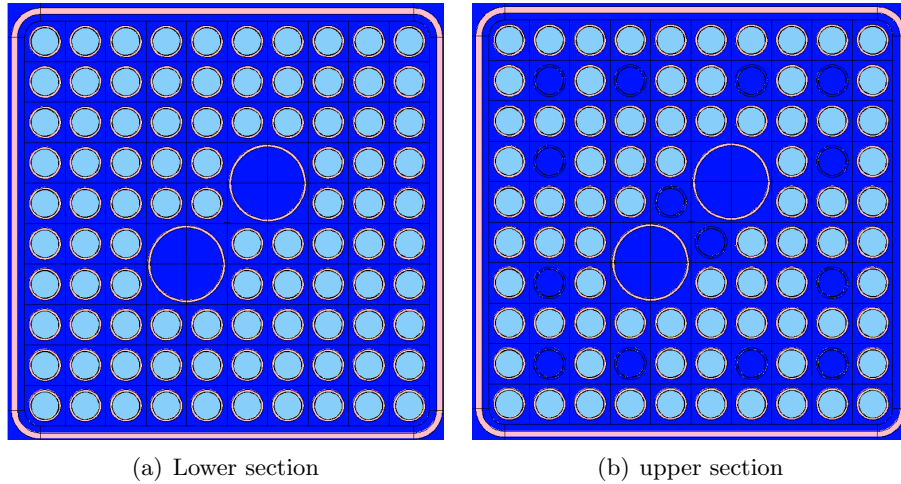
Figure 3.7: Cross section view of the 'GE14 Nordic' fuel bundle design model for O3 obtained using MCNP
