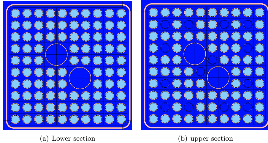
Figure 3.2: Cross section view of the 'GE14 Nordic' fuel bundle design model for O1 obtained using MCNP
