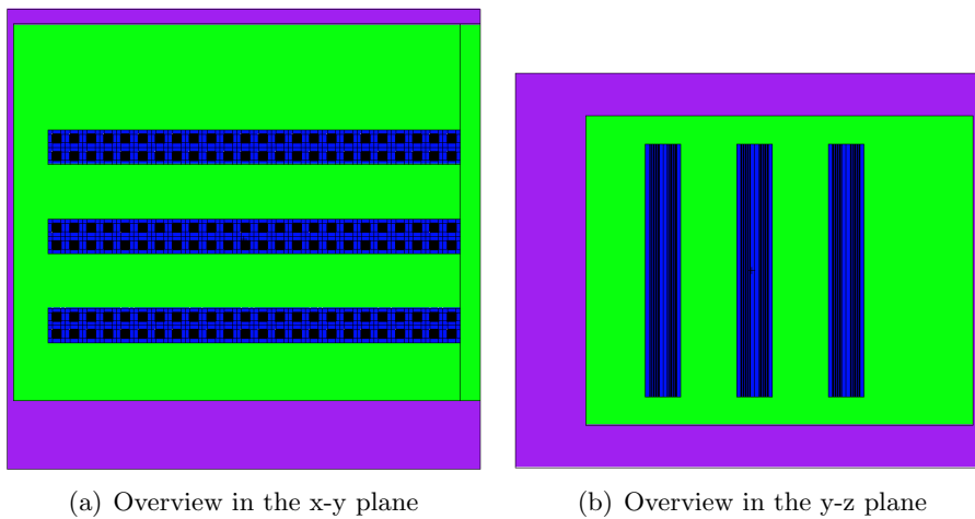
Figure 3.1: Plots of the dry storage facility model for O1 obtained using MCNP
