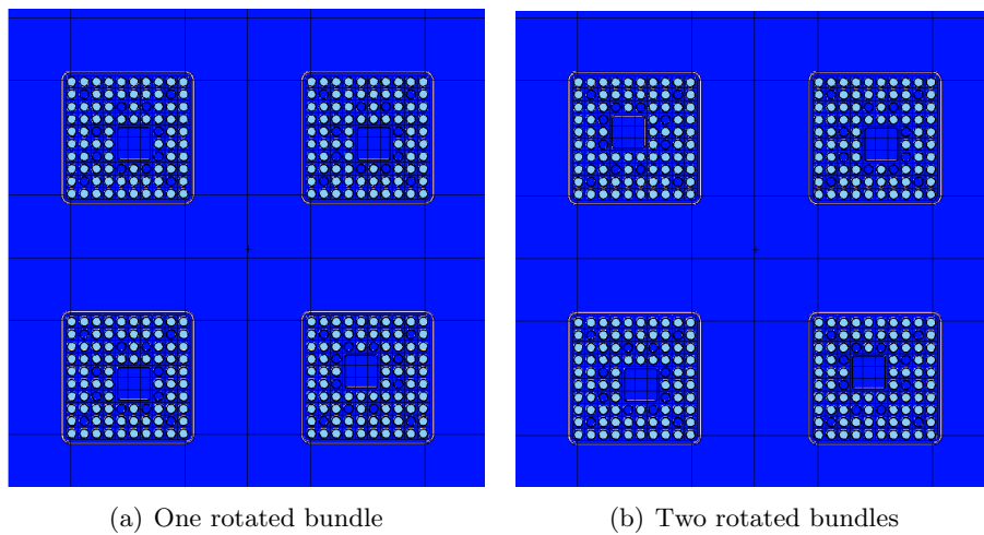
Figure 4.4: Plots of the rotated fuel bundles inside O2 dry storage facility
