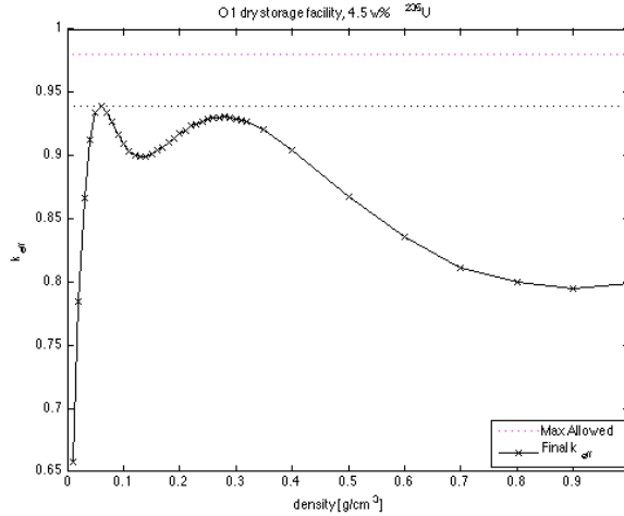
Figure 5.15: Final result of simulations of the O1 facility
