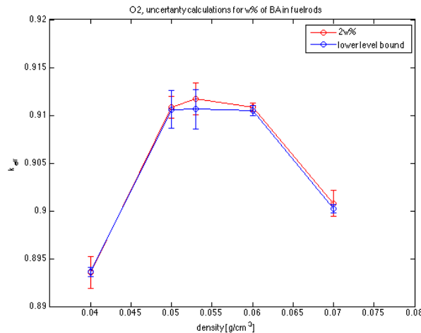
Figure 5.13: Results from simulations around optimal moderation for O2 with vendor supplied uncertainty in BA level present in pellet
