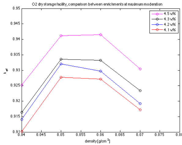
Figure 5.2: Results from simulations around optimal moderation for O2 with different enrichment levels
