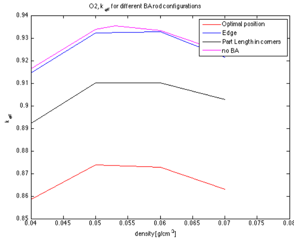
Figure 5.20: Results from the simulations of BA rod positioning
