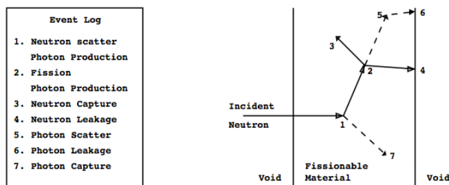
Figure 2.1: Schematic picture of a possible neutron "history" in a Monte Carlo simulation [1]
