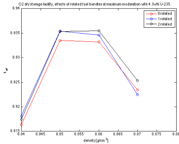
Figure 5.5: Results from simulations around optimal moderation for O2 with rotated fuel bundles
