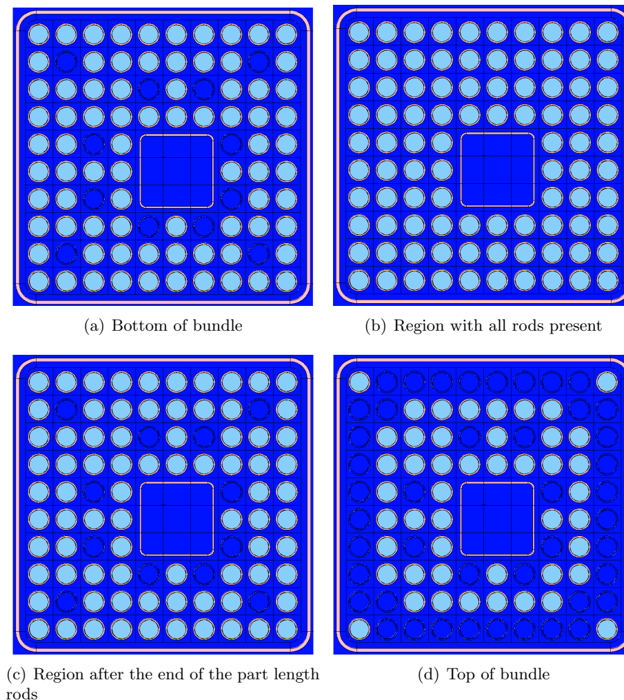
Figure 3.4: Cross section view of the 'Atrium 10XM' fuel bundle design model for O 2 obtained using MCNP
