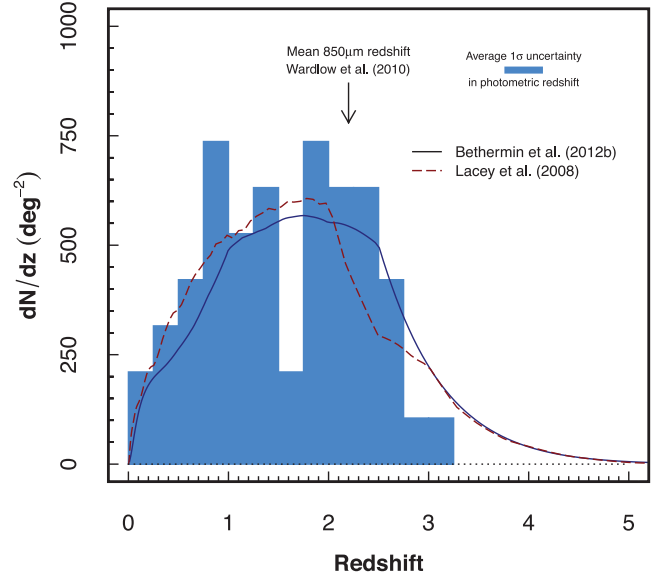
Figure 5. Redshift distribution of 54/60 450- \mu\text{m} -selected SMGs in our sample (not corrected for completeness), derived from 13-band photometric redshift estimates (Section 3.4). The average redshift of the sample is \langle z \rangle = 1.3 , and the vast majority of the 450- \mu\text{m} -selected SMGs lie at z < 3 . For comparison, the average redshift of SMGs selected at 850 \mu\text{m} is z \approx 2.2 (Wardlow et al. 2010), indicating the efficacy at which the 450 \mu\text{m} selection samples a population of SMGs at lower redshift and therefore an important complement to any census of the dusty Universe. We compare the shape of the redshift distribution to the models of B  thermin et al. (2012b) and Lacey et al. (2008) shown in Fig. 4 for galaxies with S_{450} > 5 mJy (we have area-normalized both model distributions, since the observed redshift distribution contains no completeness correction). The average redshift and shape of both model distributions is in good agreement with observations, suggesting that – at this flux limit – there is little contribution from galaxies at z > 3 .
