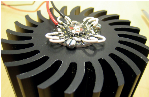
Figure 33. The multi chip fastened on a heat sink using screws.
