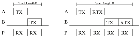
Figure 1: Schedules without Network Coding (0 and 1 retransmissions)
