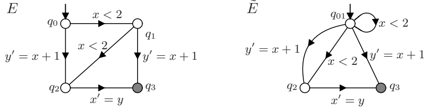
Figure 3: Example of Active Events Rule.
