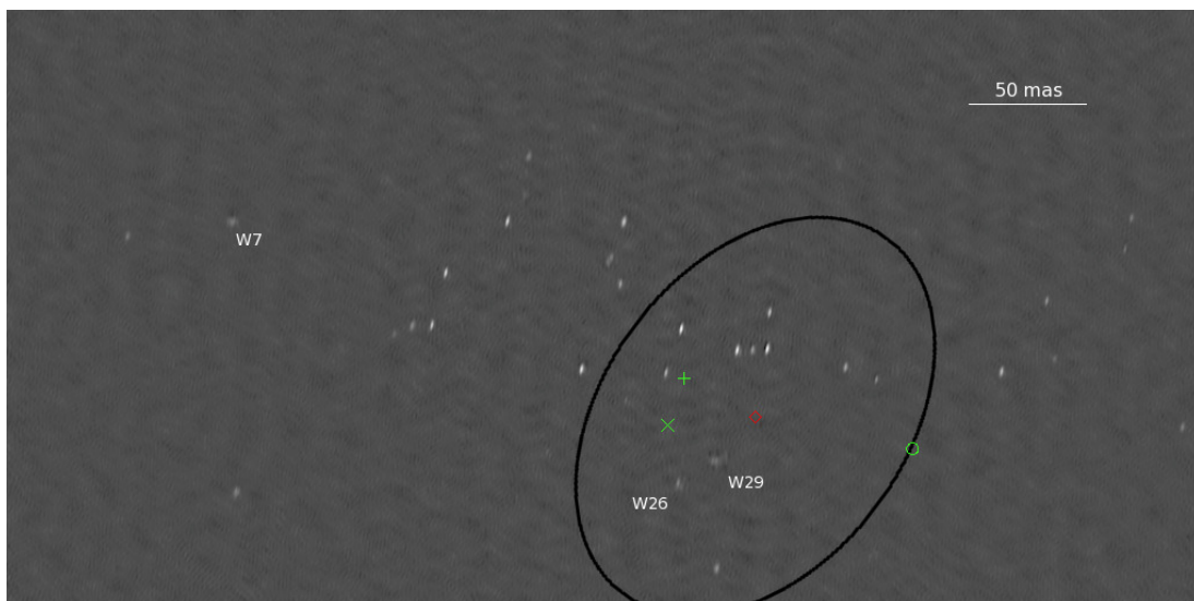
Fig. 1. Greyscale shows the combined 5 GHz global array GC031A, B, C natural weighted image of the Western nucleus. The noise rms is 8 \mu\text{Jy}/\text{beam} , the image size is 512 \times 256 mas. Labelled in white are the variable sources W7, W26 and W29. The green crosses give the 1.3 mm and 2.6 mm IRAM positions of the hot dust “AGN” feature from Downes & Eckart (2007), the green circle is the position from the 0.8 mm observation of Sakamoto et al. (2008). Errors on these positions are estimated to be of order 50–100 mas. The black ellipse gives the orientation and size of the hot dust feature as fitted by Downes & Eckart (2007) centred at the centroid (red square) of the three millimeter interferometer positions.
