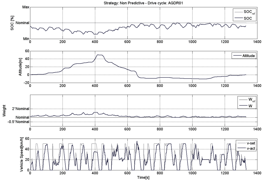
Figure 13: Short intercity drive cycle with the non predictive EMS.
