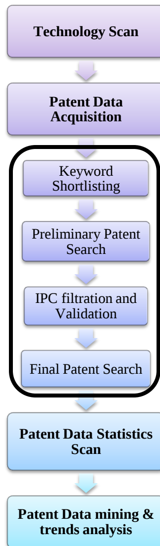
Fig1: Research Methodology
