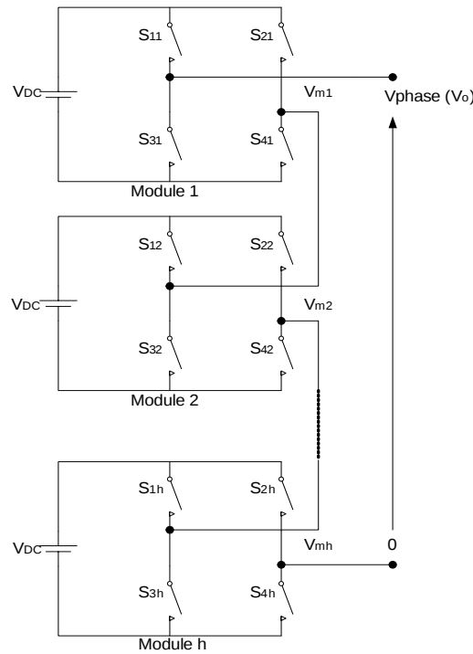
Figure 10. One phase of a cascaded H-bridge multilevel inverter
