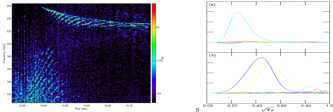
Figure 1: Left: Magnetic spectrum of the plasma center during shot 66203 on JET, measured by O-mode interferometry diagnostics. Both tornado modes and cascading modes are clearly visible. Right: Mode structure of (a) cascading mode with q_0 = 0.95 and (b) tornado mode with q_0 = 0.91 obtained numerically using MISHKA-1.
