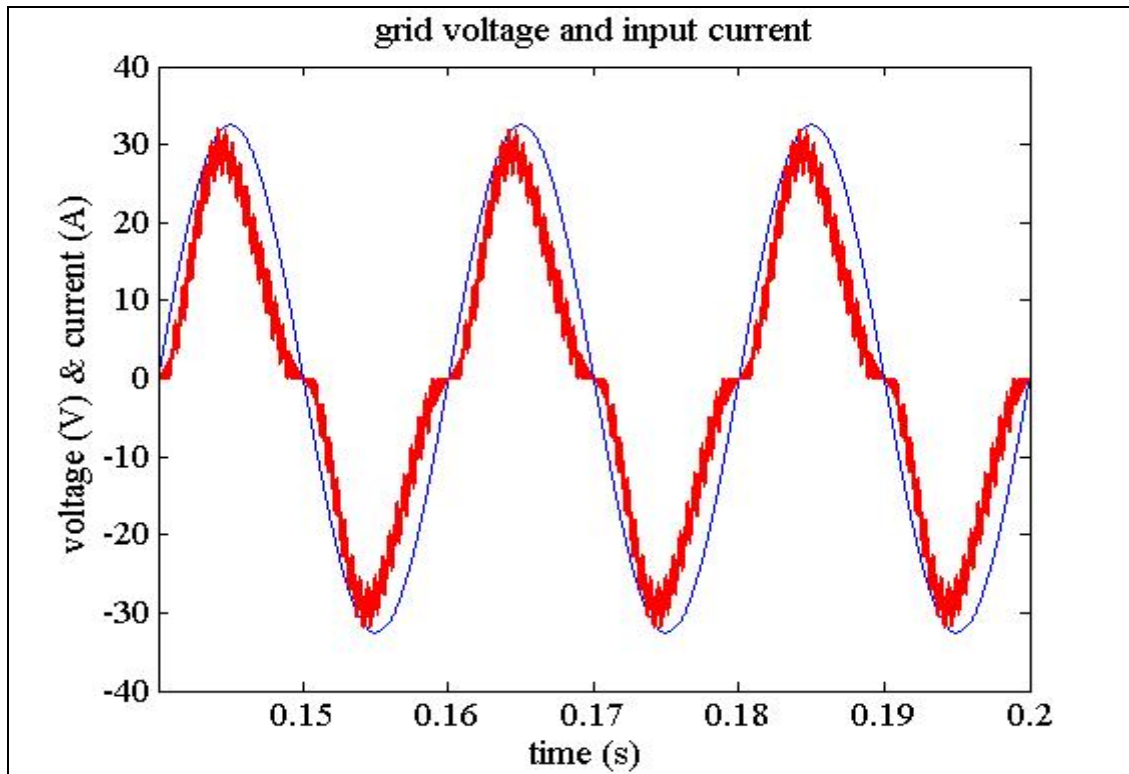
Figure 34 Input current and grid voltage
