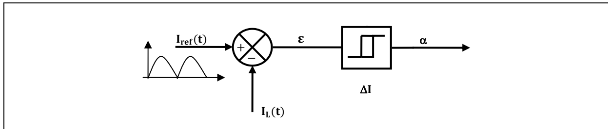
Figure 9 Current control by hysteresis
