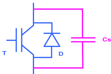
Figure 23 Capacitor snubber
