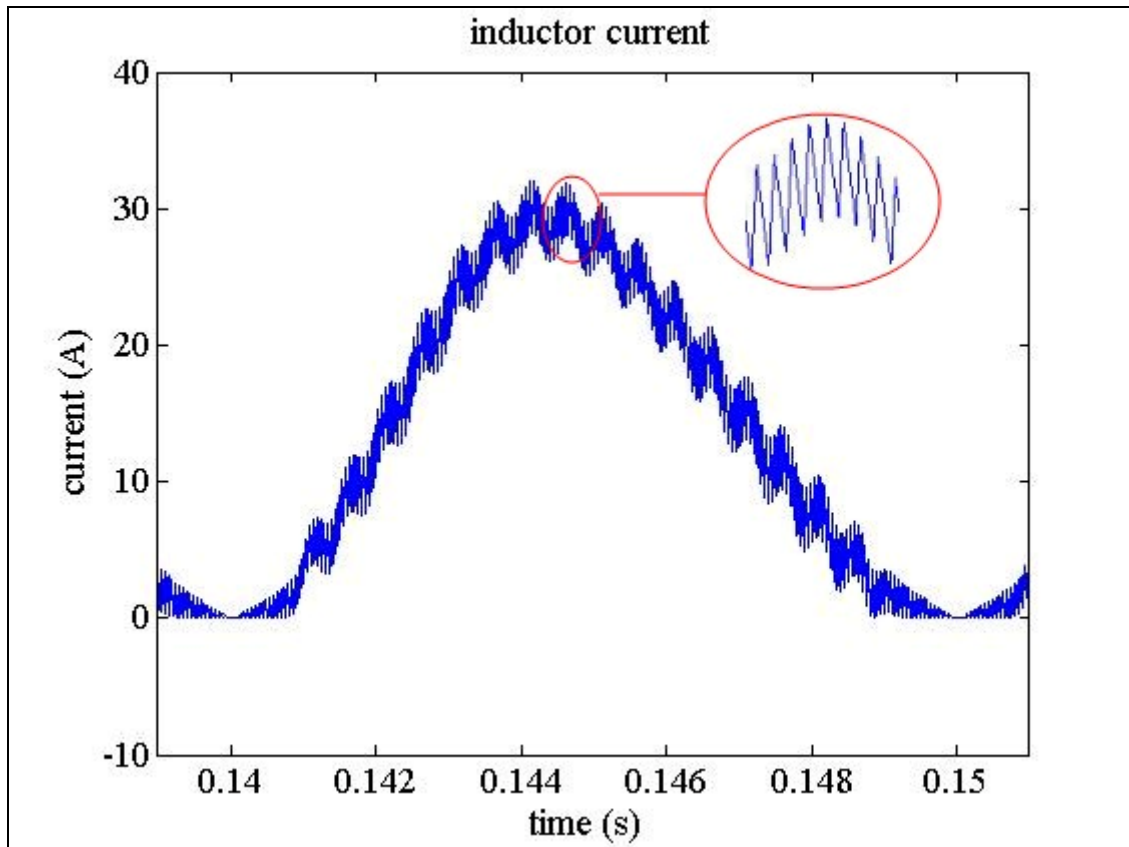
Figure 36 Inductor current
