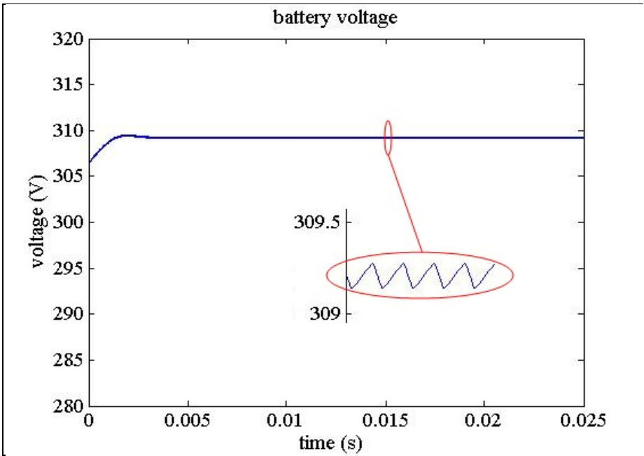
Figure 47 Voltage in the battery
