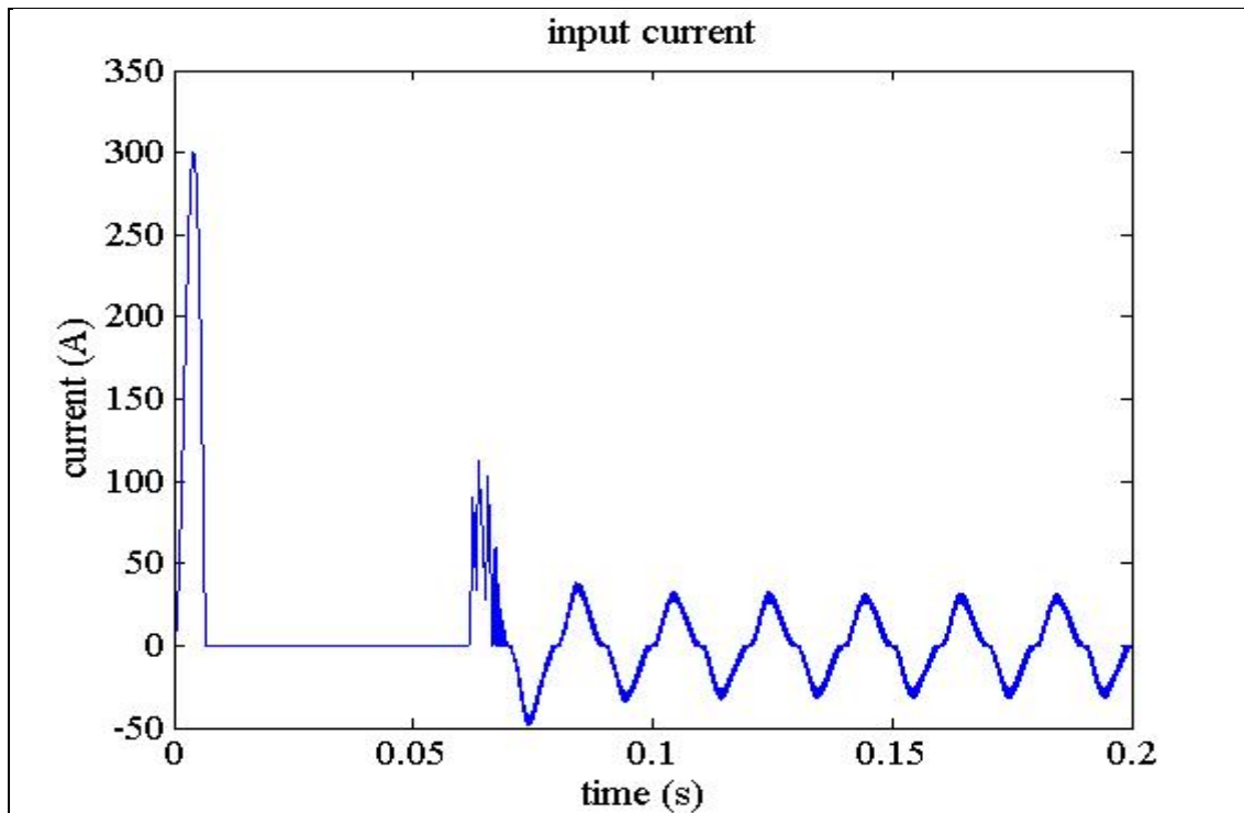
Figure 31 Input current
