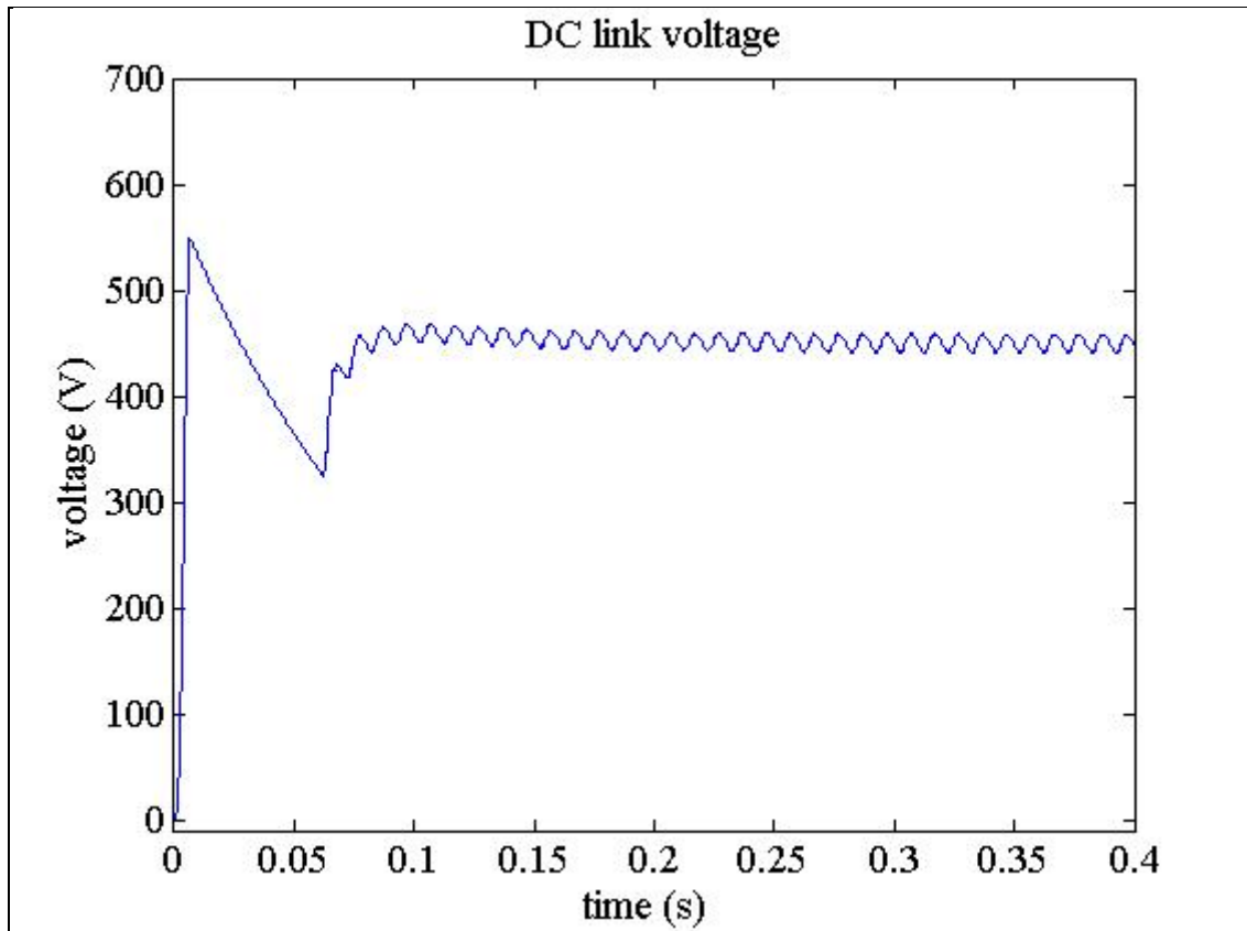
Figure 37 DC link voltage
