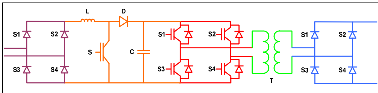
Figure 2 Power part of the on board charger
