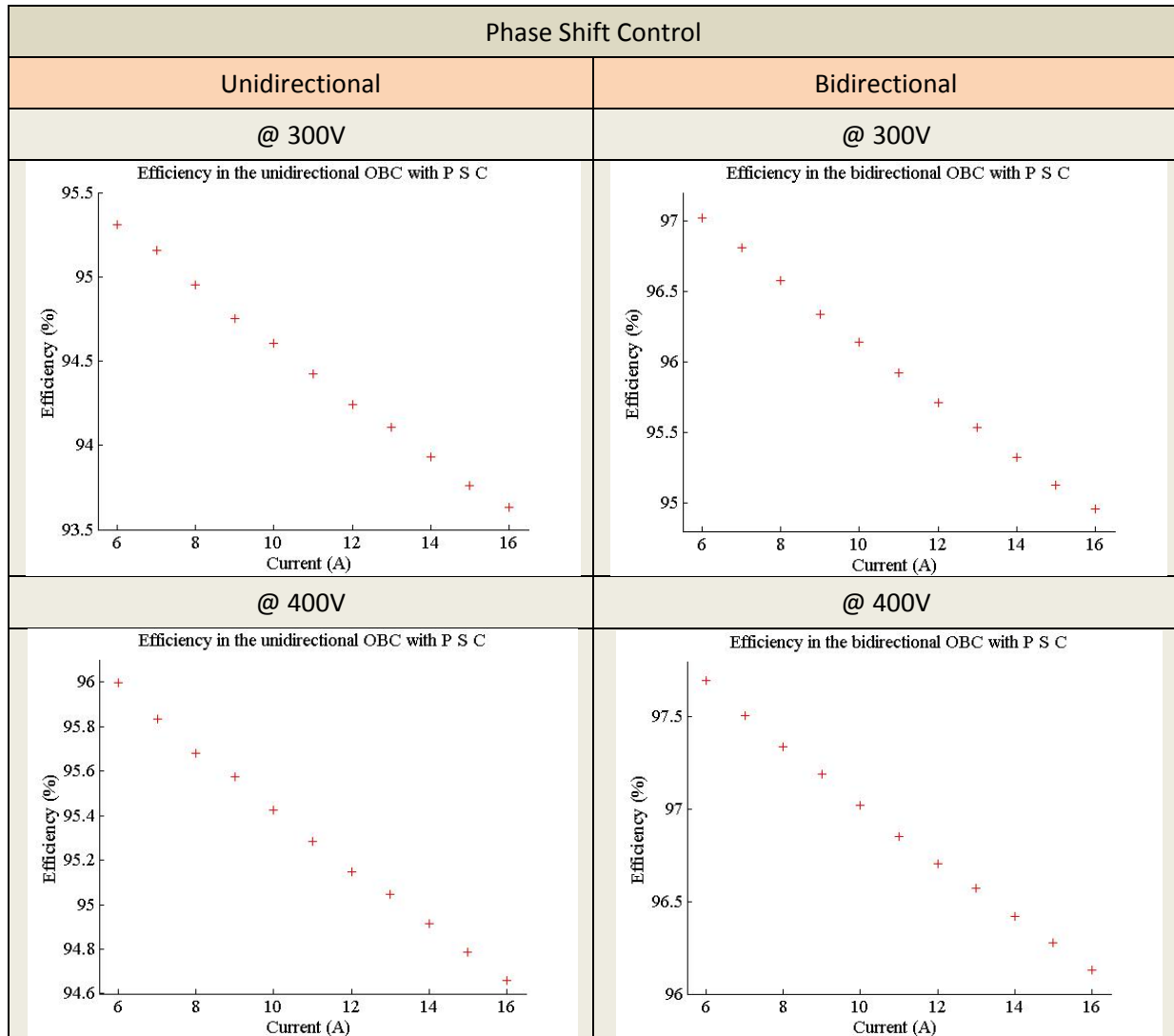
Figure 73 Efficiency comparison between bidirectional and unidirectional OBC
