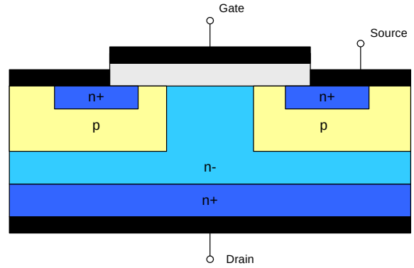
Figure 19 MOSFET structure
