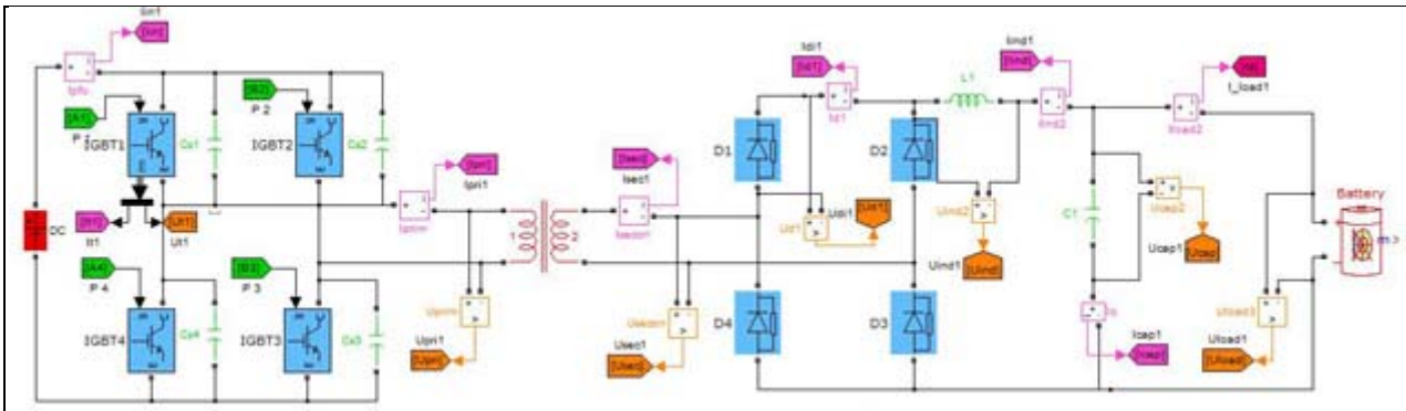
Figure 38 Power part of the full bridge converter
