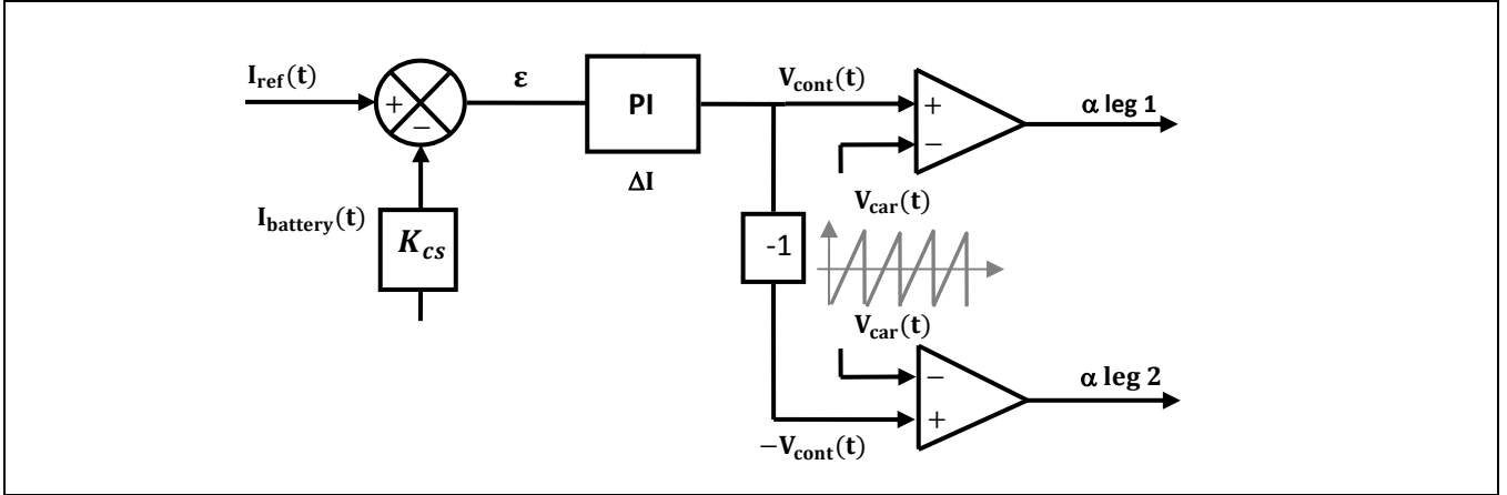
Figure 25 Current loop with phase shift control
