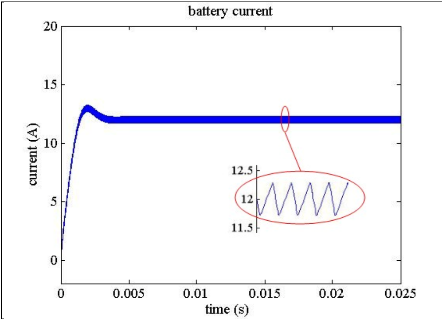
Figure 46 Current in the battery
