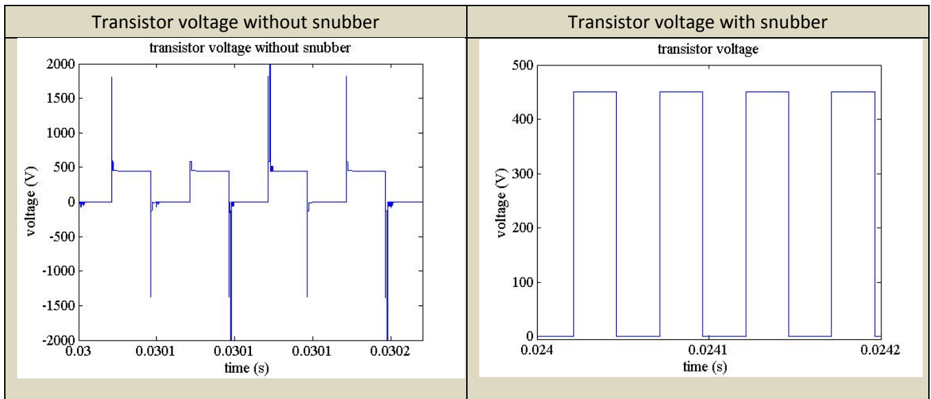
Figure 41 Role of the snubber on the transistor voltage
