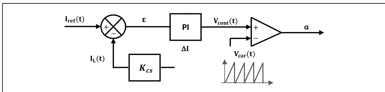
Figure 10 Current control by PWM
