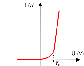
Figure 21 Current/voltage diode characteristic
