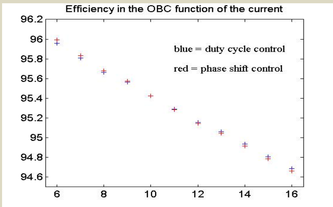
Figure 72 Efficiency of the OBC function of the control method at 400V
