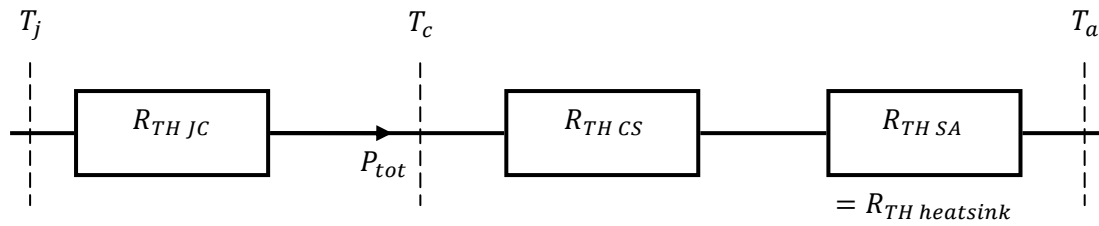
Figure 74 Thermal resistance in a system semiconductor/sink
