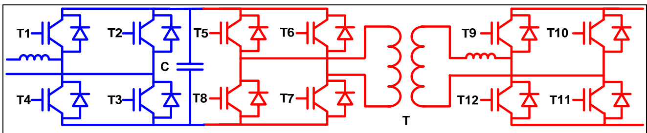
Figure 28 Power part of the bidirectional on board charger
