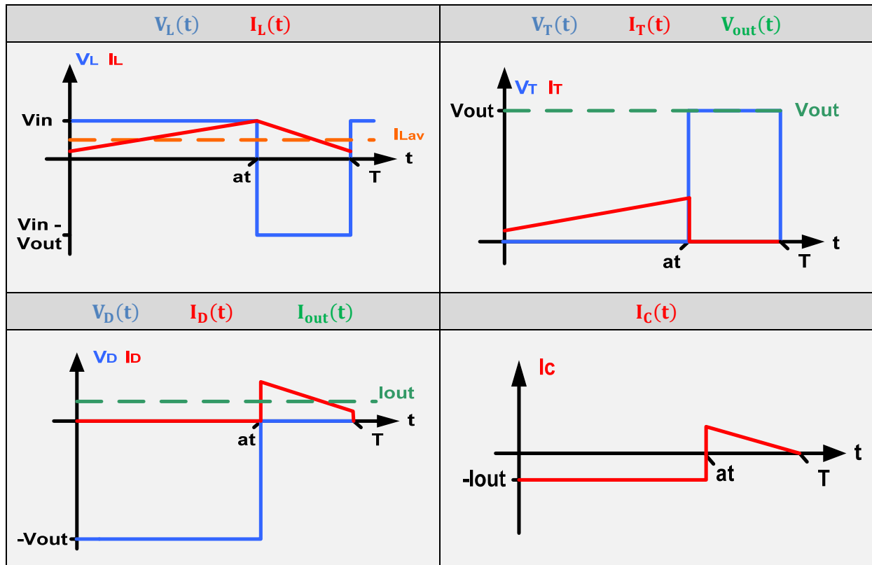
Figure 8 Current and voltage waveform in the boost converter
