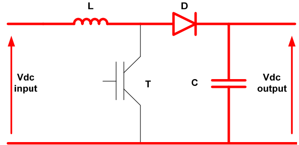
Figure 7 Current during the second phase
