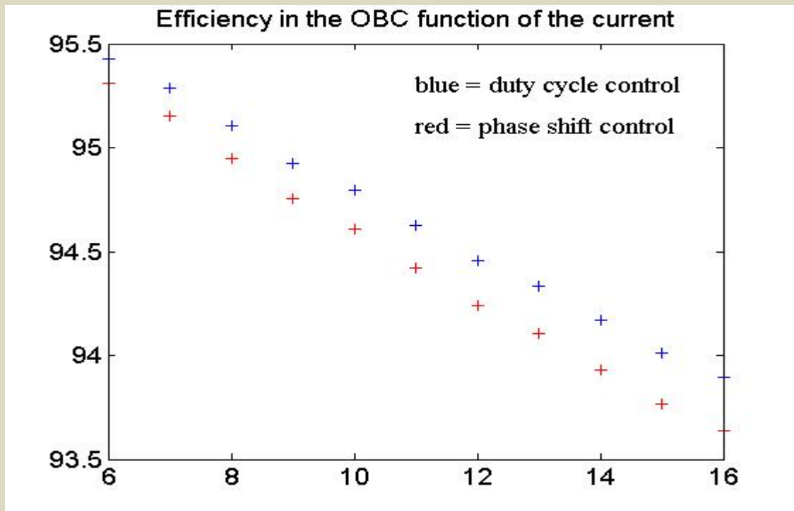
Figure 71 Efficiency of the OBC function of the control method at 300V
