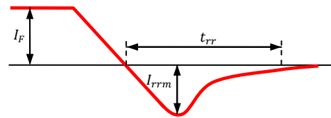
Figure 22 reverse recovery time phenomenon
