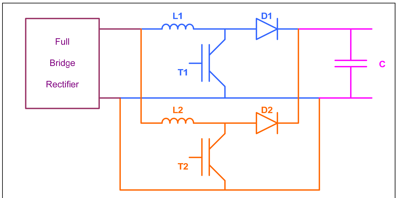
Figure 12 Two phases PFC
