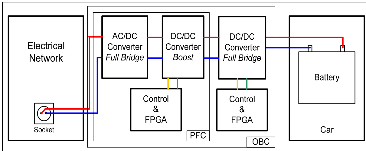
Figure 1 General diagram of the on-board charger
