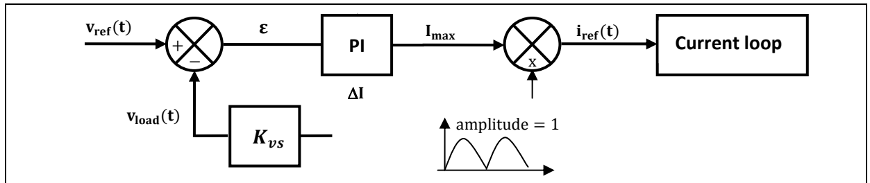
Figure 11 Voltage control
