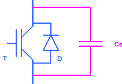
Figure 48 Snubber capacitor
