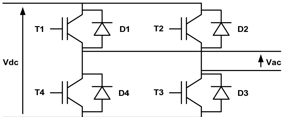
Figure 14 Full bridge inverter
