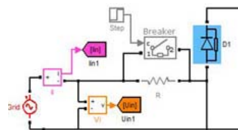
Figure 32 In rush current solver
