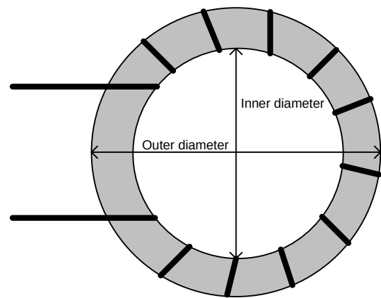
Figure 50 Shape of the inductor
