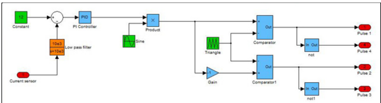
Figure 39 Control part of the full bridge converter
