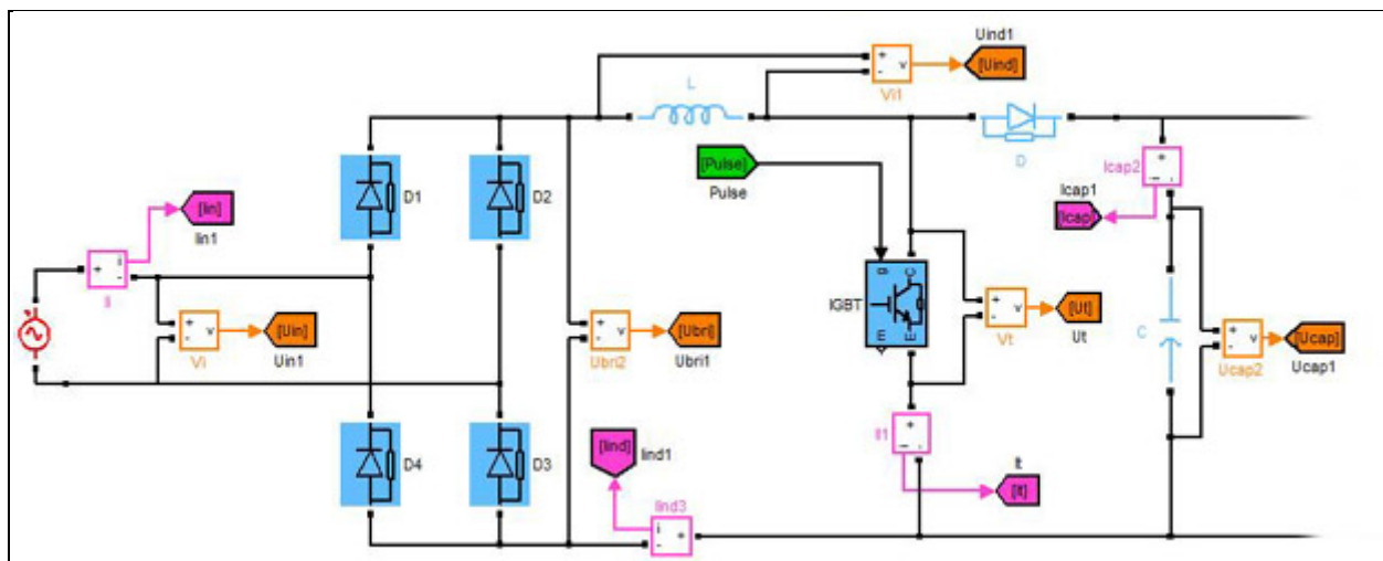
Figure 29 Power part of the PFC
