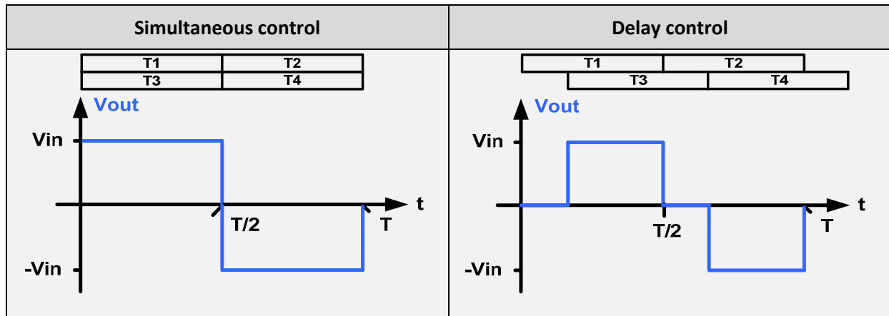
Figure 15 Output voltage according to the control method
