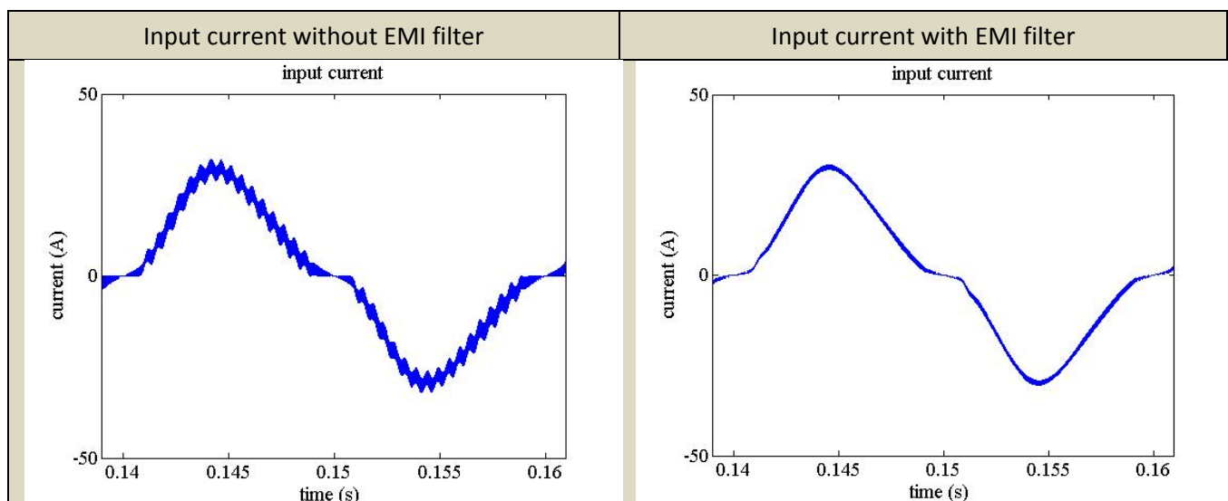
Figure 35 Role of the EMI filter
