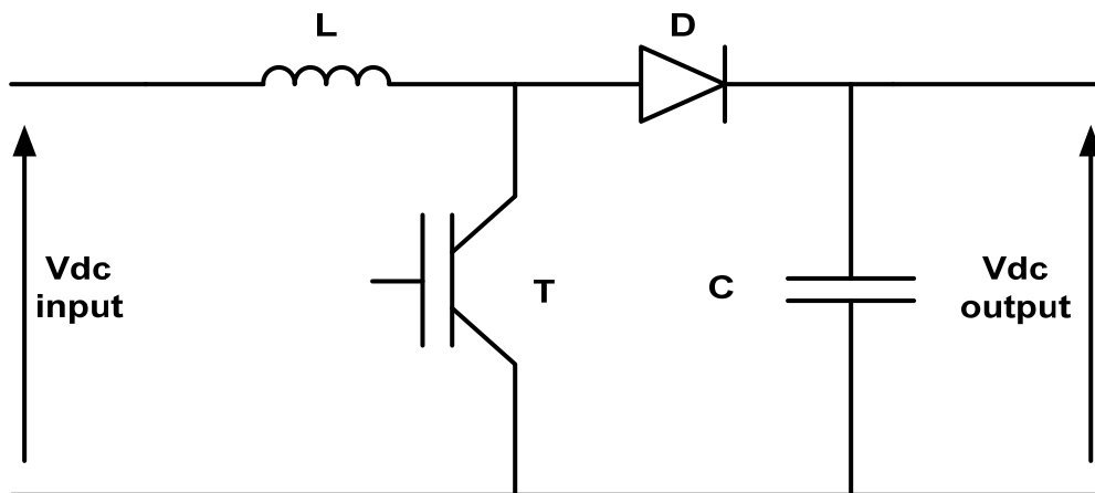
Figure 5 Boost converter
