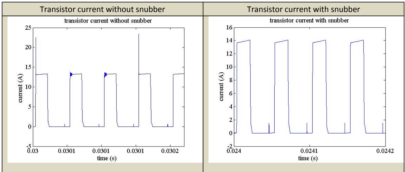
Figure 40 Role of the snubber on the transistor current
