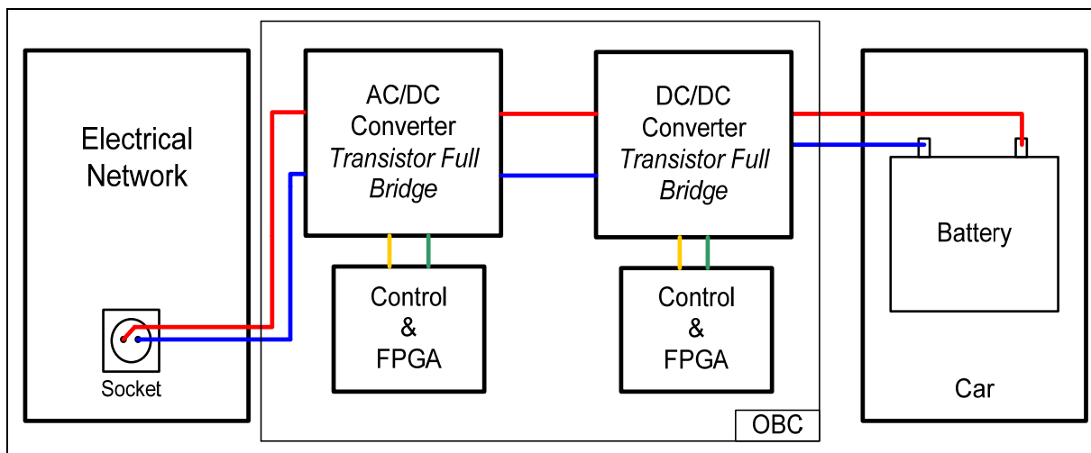
Figure 27 General diagram of the bidirectional on board charger
