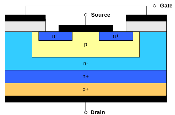
Figure 17 IGBT structure
