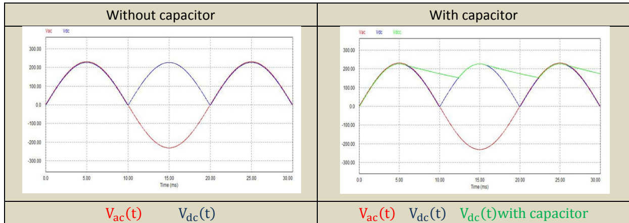
Figure 4 Bridge output voltage
