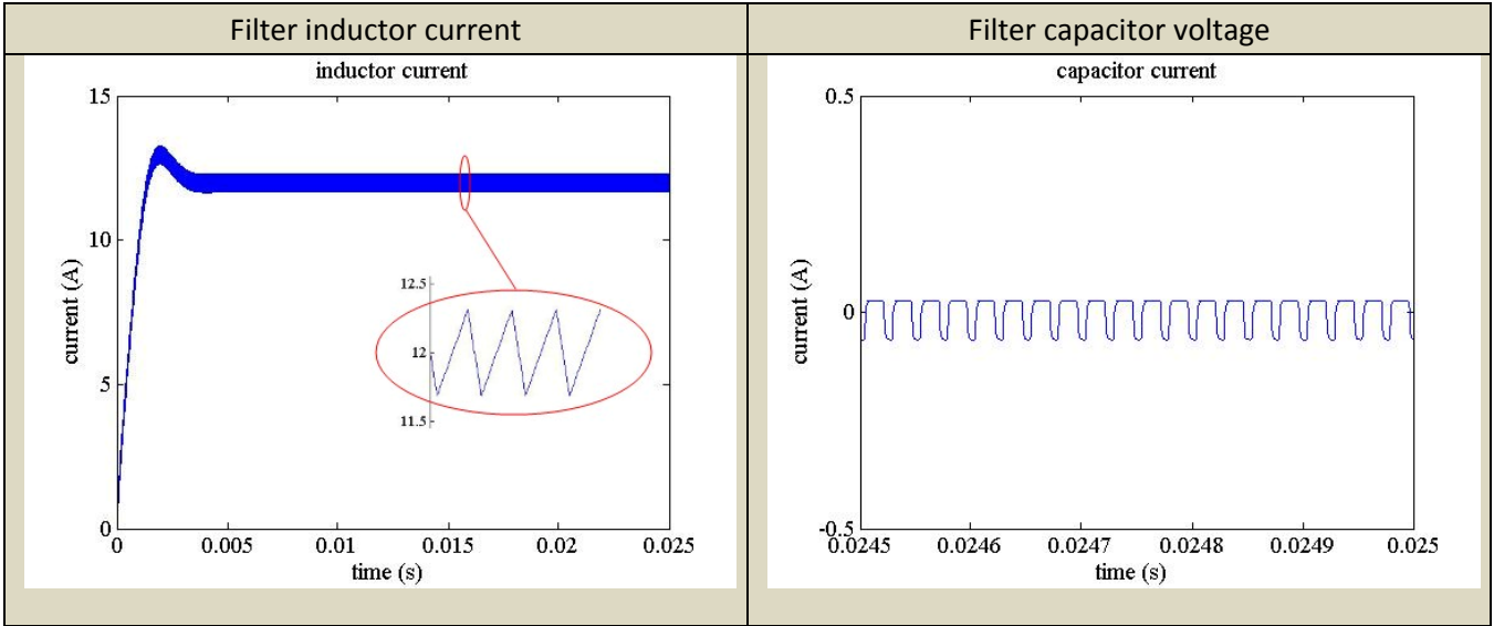
Figure 44 Inductor current
