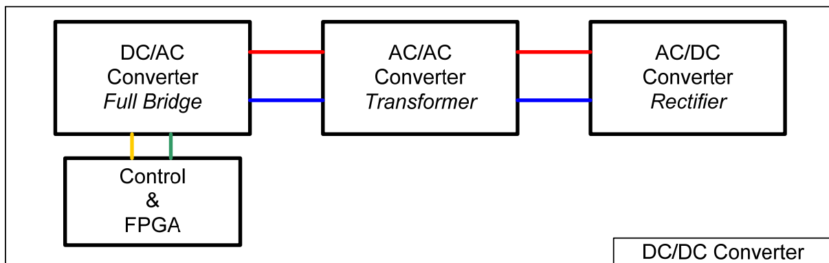
Figure 13 Structure of the full bridge converter
