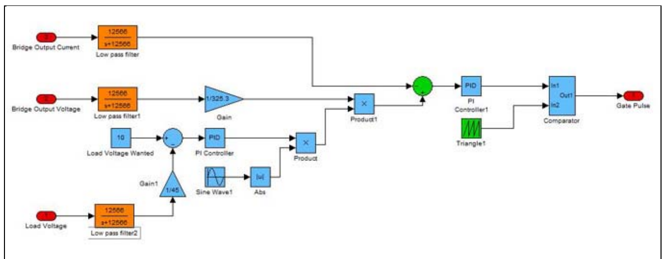
Figure 30 Control part of the PFC
