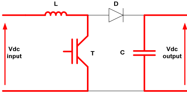
Figure 6 Current during the first phase
