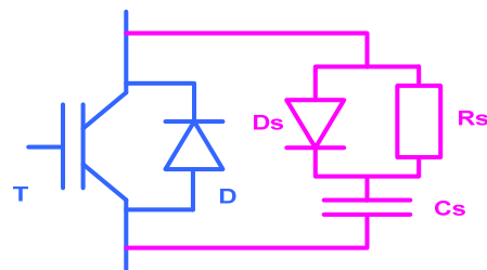
Figure 24 Resistor, capacitor and diode snubber
