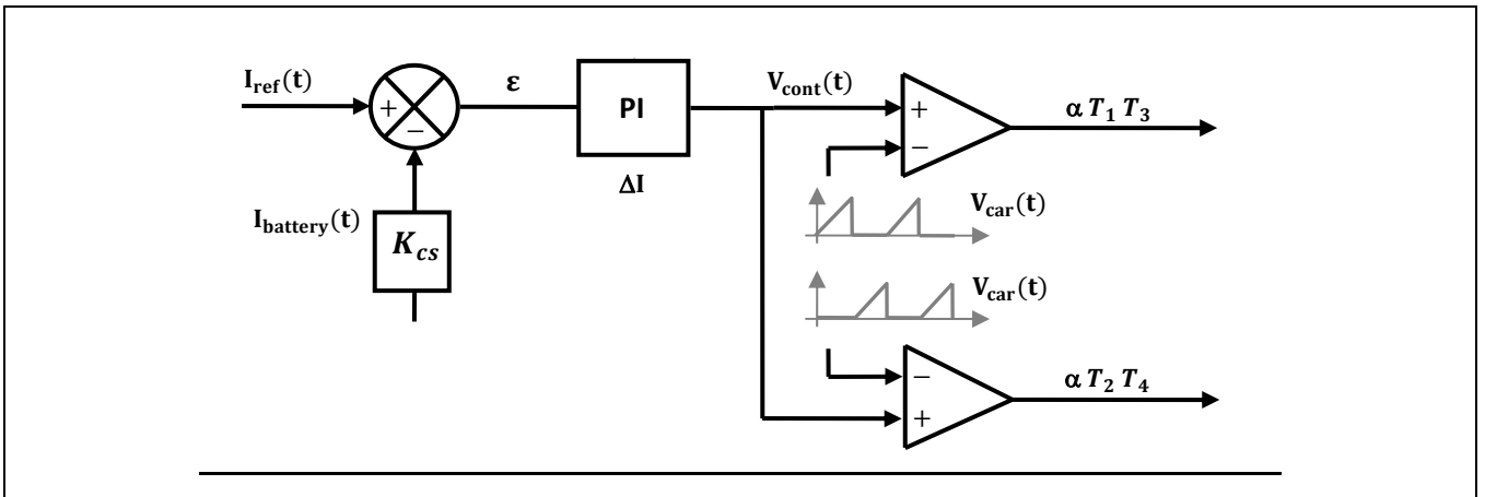
Figure 26 Current loop with duty cycle control
