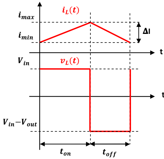
Figure 1 Current and voltage in the inductor
