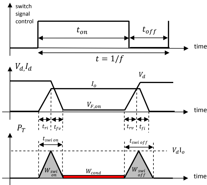
Figure 20 Current and voltage in the transistor
