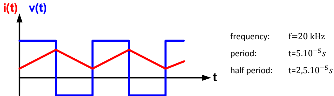
Figure 52 Current and voltage in the inductor
