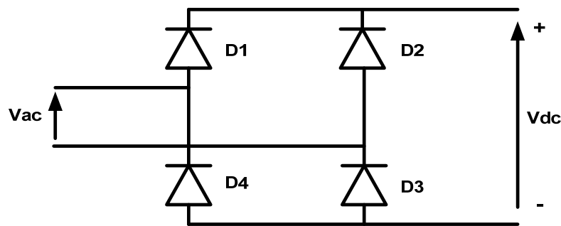
Figure 3 Diode rectifier input bridge
