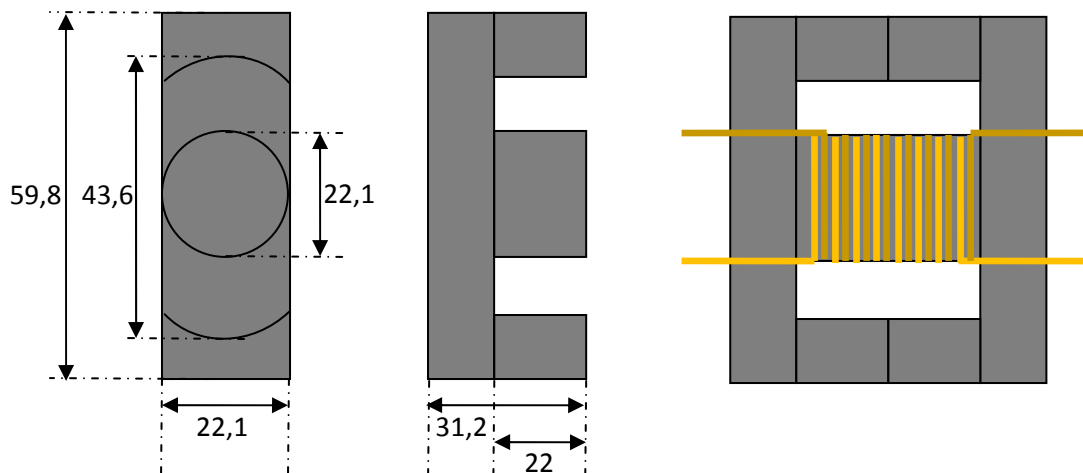
Figure 49 Size and shape of the core material
